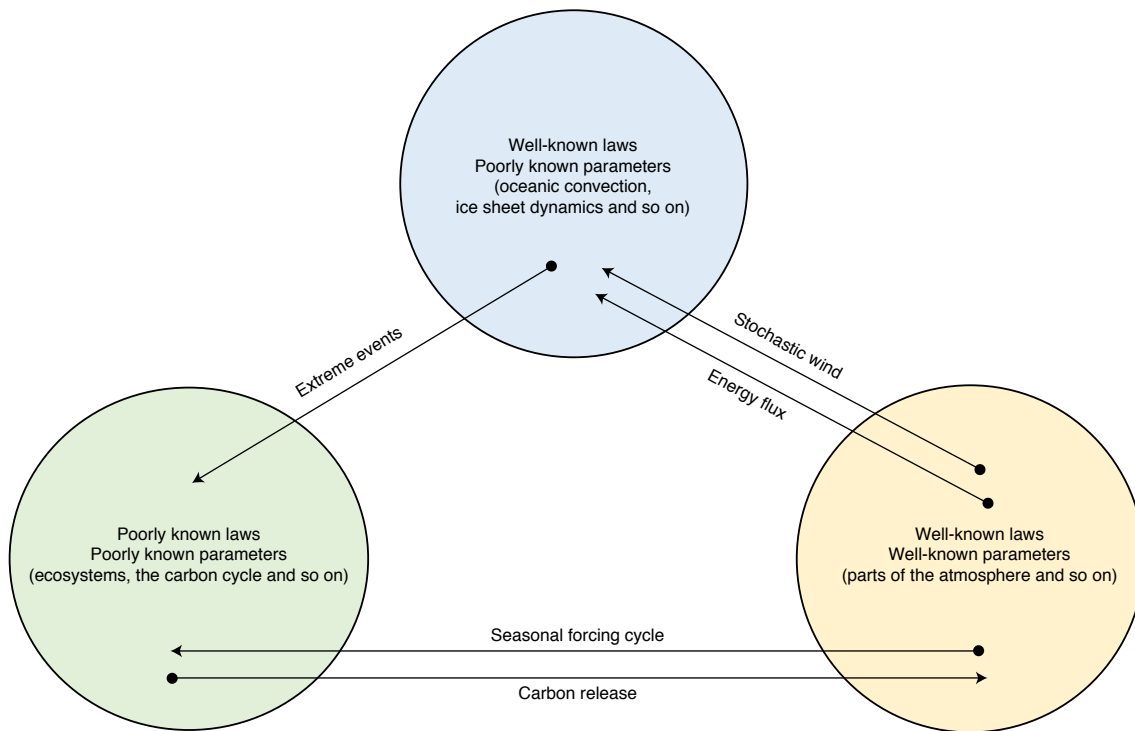
Fig. 1 | Symbolic representation of Earth system components in terms of knowledge clusters. Arrows indicate exemplary exchange of information between the clusters in terms of geophysical processes and coupling mechanisms. ML can take over different tasks depending on the cluster application; for example, data exploration and analysis in case of poor process knowledge (green cluster), ESM enhancement by improving insufficient parameterizations and other simplifications in process-based models (blue cluster) or emulation and acceleration of well-understood process-based simulations (orange cluster). Similarly, ML can be applied to coupling mechanisms and interaction processes (arrows), utilizing adjacent clusters as training data pools.
