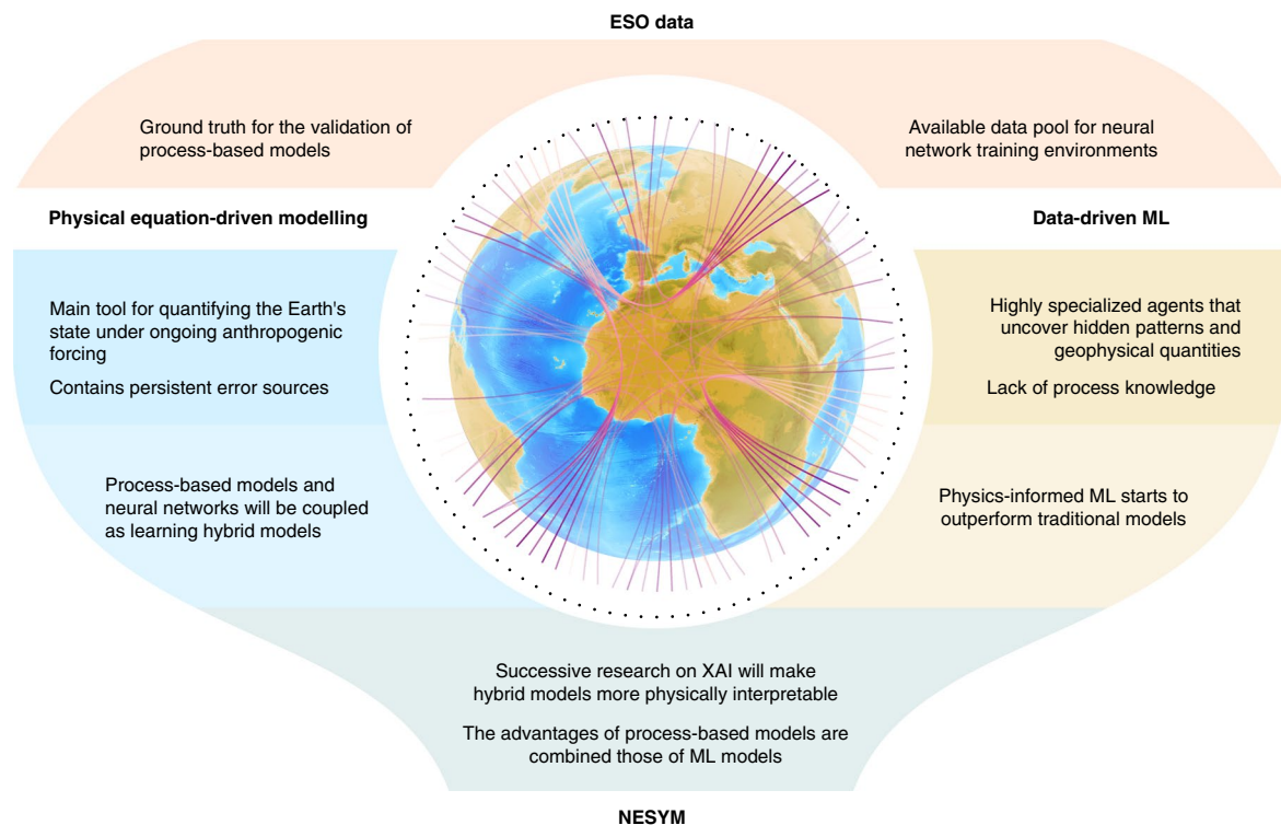
Fig. 2 | Successive stages of the fusion process of ESMs and AI towards NESYM. The left and right branches visualize the current efforts and goals for building weakly coupled hybrids (blue and yellow), which converge towards strongly coupled hybrids with support from XAI. More details of weak and strong hybrids are provided in the text.
