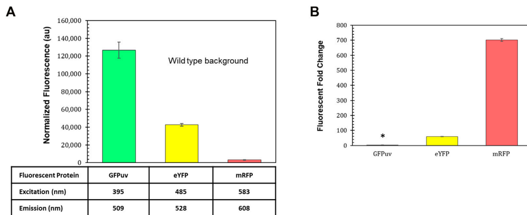
FIGURE 2 | Fluorescent reporters and background fluorescence. (A) Average fluorescence of wild type R. palustris normalized to absorbance (660 nm), in triplicate, at the emission and excitation wavelengths for GFPuv, eYFP, and mRFP (Materials and Methods). Error bars represent the population standard deviation. (B) Fluorescent fold change average of R. palustris BBR1-kan-GFPuv, BBR1-kan-eYFP, and BBR1-kan-mRFP strains grown in triplicate. 300 µg/ml kanamycin sulfate was added to the media for the mutant strains but not wild type R. palustris (Materials and Methods). * indicates statistically significant expression of 3-fold for the BBR1-kan-GFPuv strain. Error bars represent the population standard deviation.
