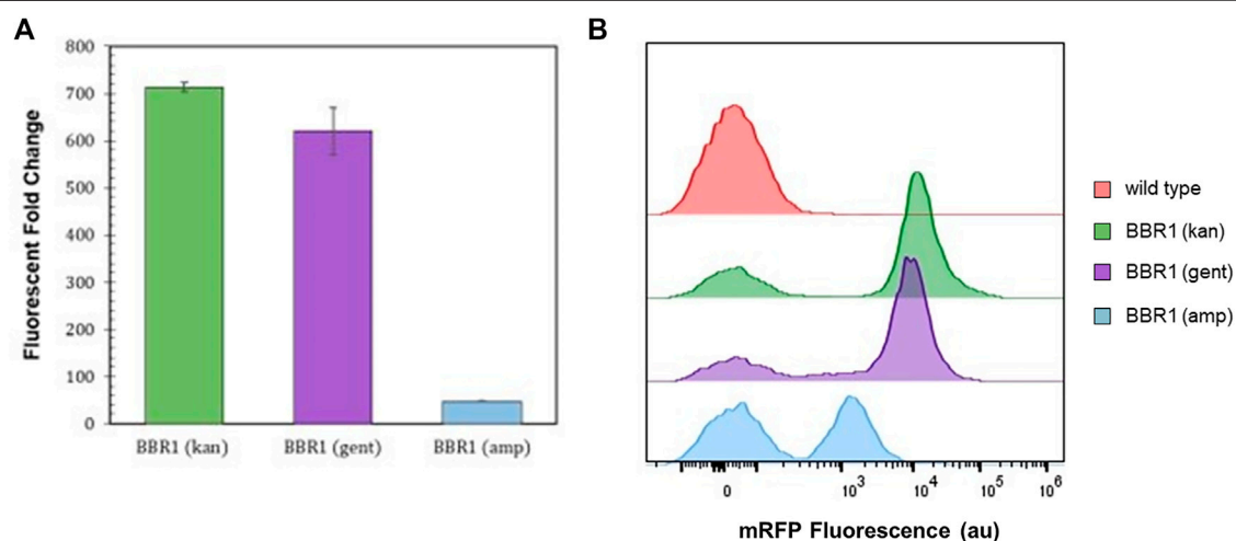
FIGURE 3 | Expression tests and flow cytometry results (A) Average fluorescent fold change of R. palustris BBR1-kan-mRFP, BBR1-gent-mRFP, and BBR1-amp-mRFP strains grown in triplicate. The antibiotic concentrations added to the media of the mutant strains but not wild type R. palustris were 300 µg/ml kanamycin sulfate, 300 µg/ml gentamicin sulfate, and 50 µg/ml ampicillin respectively (Materials and Methods). Error bars represent the population standard deviation. (B) Representative flow cytometry results of mRFP fluorescence from R. palustris wild type, BBR1-kan-mRFP, BBR1-gent-mRFP, and BBR1-amp-mRFP strains grown in triplicate. The growth procedure, media, and antibiotics are the same as for the fluorescent fold change test in Figure 3A (Materials and Methods).
