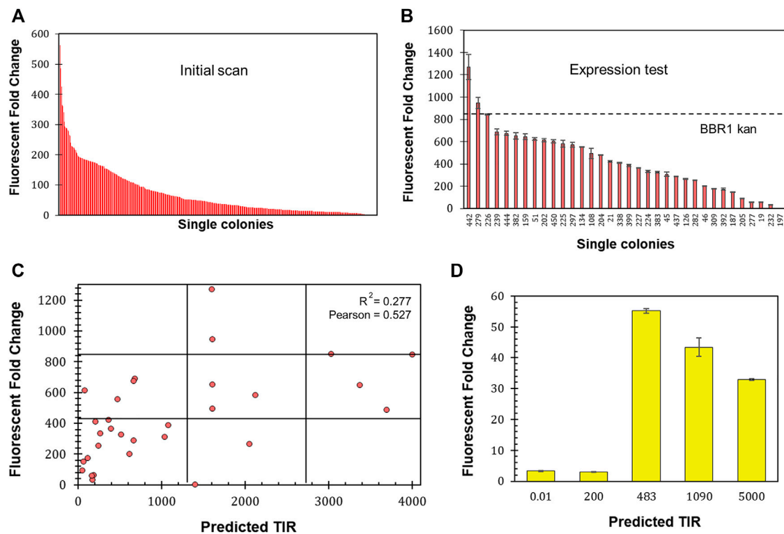
FIGURE 7 | Determining 5' UTR design guidelines for R. palustris . (A) Fluorescent fold change scan of R. palustris BBR1-kan-mRFP (RBS library) single colonies (Materials and Methods). (B) Average fluorescent fold change of select R. palustris BBR1-kan-mRFP (RBS library) strains grown in triplicate (Materials and Methods). Error bars represent the population standard deviation. (C) Comparison of the predicted translation initiation rate (TIR) versus the fluorescent fold change average of the select R. palustris BBR1-kan (RBS library)-mRFP strains. The grid lines divide each axis in thirds to aid in analysis. (D) Average fluorescent fold change of R. palustris BBR1-kan (0.01, 200, 483, 1,090, and 5,000)-5' UTR-eYFP strains grown in triplicate (Materials and Methods). Error bars represent the population standard deviation.
