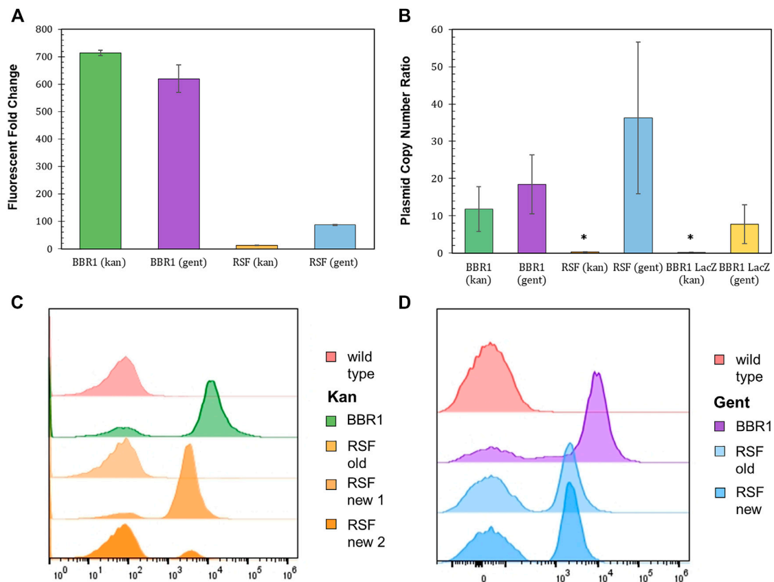
FIGURE 4 | Origin of replication characterization with different selection markers and reporters. (A) Fluorescent fold change average of R. palustris BBR1-kan-mRFP, BBR1-gent-mRFP, RSF1010-kan-mRFP, and RSF1010-gent-mRFP strains grown in triplicate. The antibiotic concentrations added to the media of the mutant strains but not wild type R. palustris were 300 \mu g/ml kanamycin sulfate and 300 \mu g/ml gentamicin sulfate respectively (Materials and Methods). Error bars represent the population standard deviation. (B) Average plasmid copy number for the R. palustris BBR1-kan-mRFP, BBR1-gent-mRFP, RSF1010-kan-mRFP, RSF1010-gent-mRFP, BBR1-kan LacZ, and BBR1-gent-LacZ strains grown in at least duplicate. The antibiotic concentrations added to the media of the mutant strains were 300 \mu g/ml kanamycin sulfate and 300 \mu g/ml gentamicin sulfate respectively. Copies of the kanamycin and gentamicin selection marker gene were compared to the single copy dxs gene in the chromosome by qPCR and an external standard curve. * indicates a statistically significant plasmid copy number of less than 1, 0.34-fold for the RSF1010-kan-mRFP strain and 0.16 for the BBR1-kan-LacZ strain (Materials and Methods). Error bars represent the population standard deviation. (C) Representative flow cytometry results of mRFP fluorescence from R. palustris wild type, BBR1-kan-mRFP, and RSF1010-kan-mRFP strains grown in triplicate. The old RSF1010-kan cultures had been streaked from frozen stock 2 weeks earlier. The new RSF1010-kan cultures were single colonies from a new transformation. The growth procedure, media, and antibiotics are the same as for the fluorescent fold change test in Figure 4A (Materials and Methods). (D) Representative flow cytometry results of mRFP fluorescence from R. palustris wild type, BBR1-gent-mRFP, and RSF1010-gent-mRFP strains grown in triplicate. The old RSF1010-gent cultures had been streaked from frozen stock 2 weeks earlier. The new RSF1010-gent cultures were single colonies from a new transformation. The growth procedure, media, and antibiotics are the same as for the fluorescent fold change test in Figure 4A (Materials and Methods).
