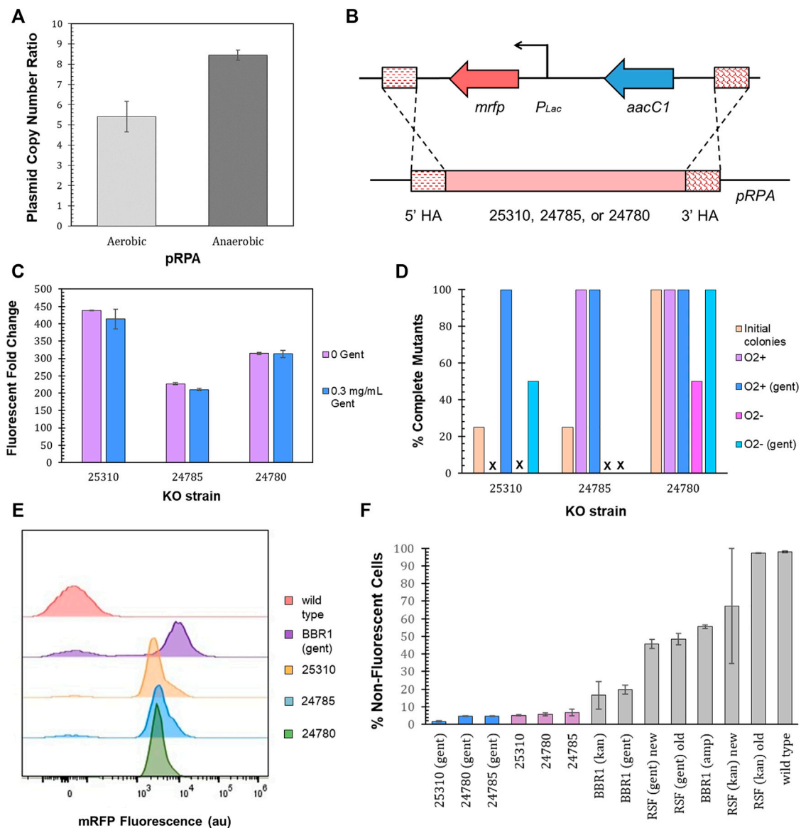
FIGURE 8 | pRPA as a heterologous gene expression vector. (A) Average pRPA copy number for wild type R. palustris grown aerobically in the dark and anaerobically in the light (100 \mu E white light) in duplicate. Copies of the plasmid's replication protein gene (TX73_RS24750) was compared to the single copy dxs gene in the chromosome by qPCR and an external standard curve (Materials and Methods). Error bars represent the population standard deviation. (B) Schematic of the P_{Lac} - mrfp expression cassette and a gentamicin selection marker integrated into one of three locations, TX73_RS25310, TX73_RS24785, TX73_RS24780, in R. palustris endogenous plasmid, pRPA, by double homologous recombination. (C) Fluorescent fold change average of R. palustris pRPA-25310-mRFP-Gent, pRPA-24785-mRFP-Gent, and pRPA-24780-Gent strains grown in triplicate either without any antibiotic or with 0.3 mg/ml gentamicin sulfate. The data is representative of the first test with new cultures as well as the test after three rounds of dilution and regrowth (Materials and Methods). Error bars represent the population standard deviation. (D) Comparison of the percent complete mutants (those that do not produce an amplicon from PCR with primers binding to the DNA that is removed and also produce the correct sequence from PCR with primers outside of the homology arms) for the three pRPA locations. (E) Representative flow cytometry results of mRFP fluorescence from R. palustris wild type, BBR1-gent-mRFP, pRPA-25310-mRFP-Gent, pRPA-24785-mRFP-Gent, and pRPA-24780-Gent strains grown in triplicate. The growth procedure, media, and antibiotics are the same as for the fluorescent fold change test in Figure 8C (Materials and Methods). (F) Average percent non-fluorescent cells for R. palustris strains grown in triplicate as determined by flow cytometry (Materials and Methods). Error bars represent the population standard deviation.
