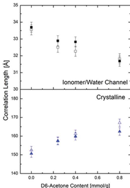
Fig. 5 SAXS correlation lengths averaged over 3 water concentrations (see Fig. S4, ESI†) as a function of acetone concentration in non-functionalized Nafion (filled points) and VA functionalized Nafion (empty points) at 296 K.
