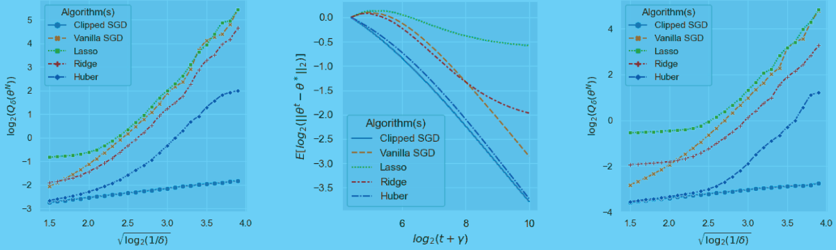
(d) Last iteration quantile loss for N = 500 and p = 20 . (e) Expected convergence curve for N = 1000 and p = 20 . (f) Last iteration quantile loss for N = 1000 and p = 20 .
