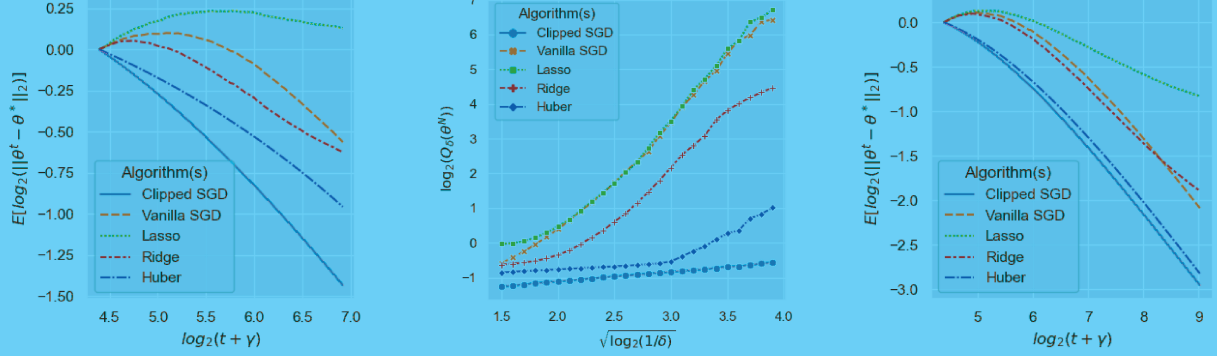
(a) Expected convergence curve for N = 100 and p = 20 . (b) Last iteration quantile loss for N = 100 and p = 20 . (c) Expected convergence curve for N = 500 and p = 20 .
