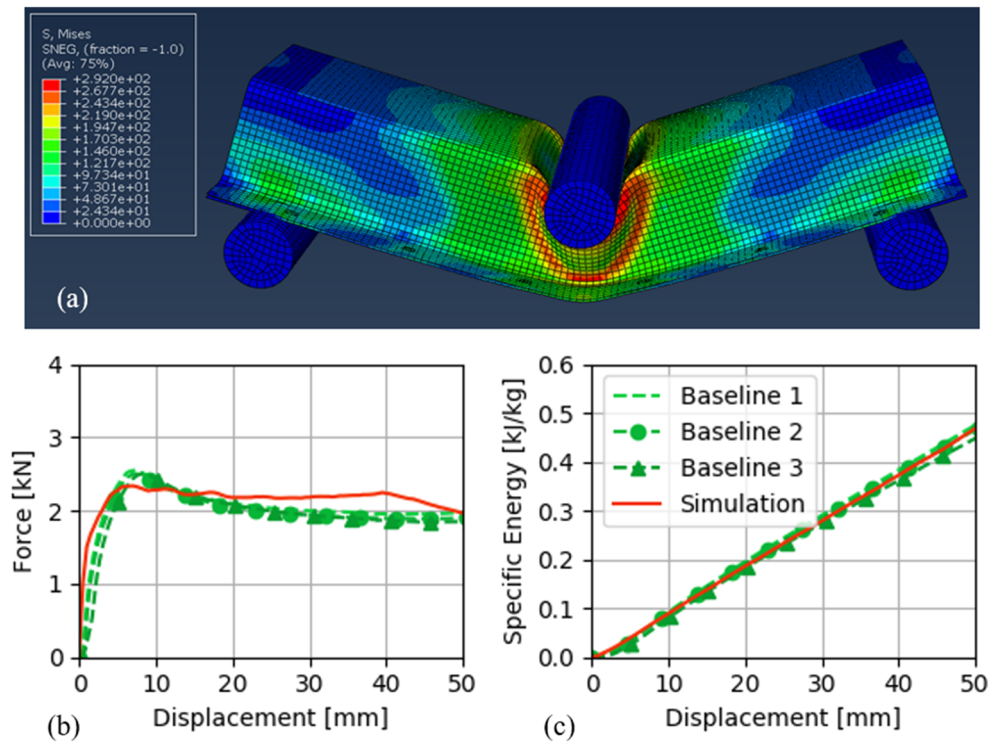
Fig. 14 Baseline model simulation result. a Deformed shape at 50 mm displacement with stress distribution, b force-displacement plot, and c SEA-displacement plot
