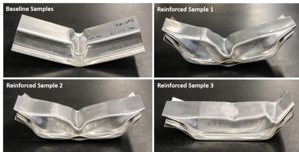
Fig. 13 Photos of tested hat-plate samples, showing representative failure modes for baseline and Al reinforced cases
