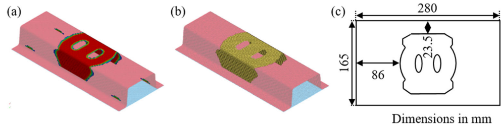
Fig. 5 Comparison of the (a) optimized reinforcement geometry, (b) generalized reinforcement geometry and (c) location of the generalized reinforcement patch on the developed blank for three-point bend specimens
