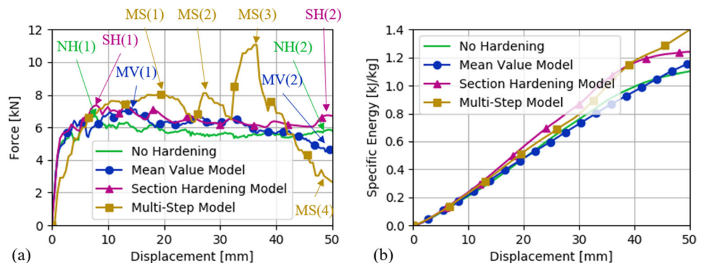
Fig. 15 Simulation results of reinforce hat section models. a Force-displacement result of each model and b specific energy absorption of each model. The indicated points represent peak loads for each model
