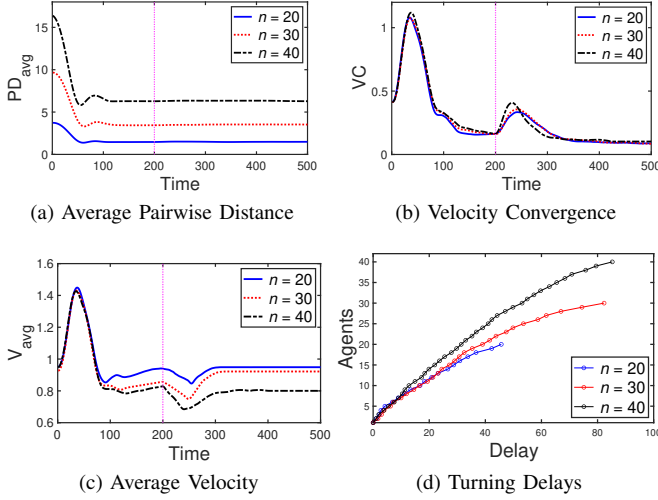
Fig. 2: Performance eval. of AWN-DMPC controller averaged over 100 runs. Turning maneuver commences at k = 200
