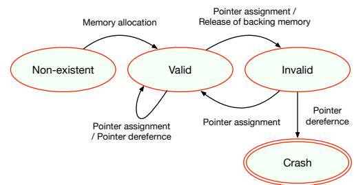
Figure 3: Pointer life-cycle
