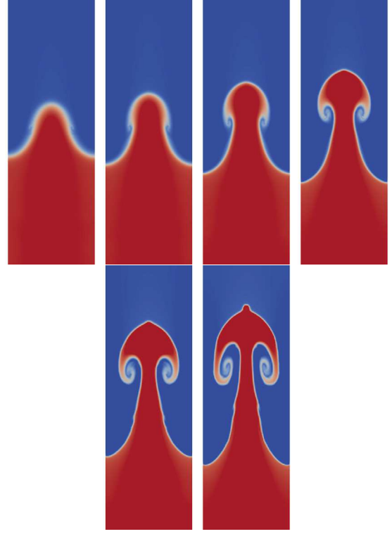
Fig. 1. Contours of the mass density at t = 1.0, 1.2, 1.4, 1.6, 1.8, 2.0 in the Rayleigh-Taylor instability simulation.
