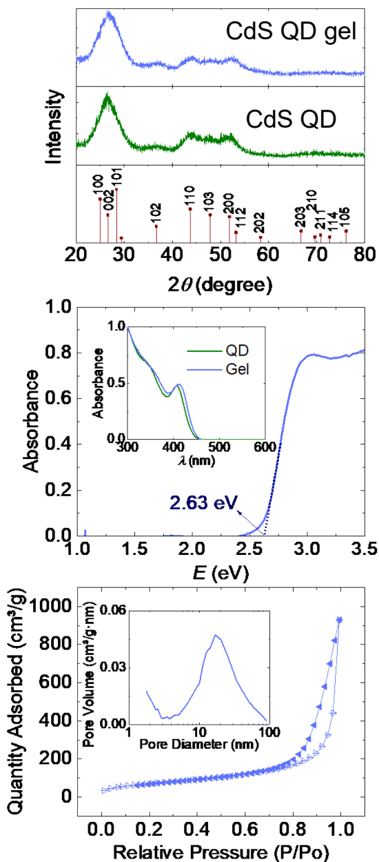
Figure 2. a, Powder X-ray diffraction (PXRD) patterns of CdS QD ME-aerogel and CdS QDs; the hexagonal CdS (wurtzite) PXRD pattern is shown as a reference (stick diagram; PDF 00-001-0780). b, Diffuse reflectance spectrum of a CdS QD ME-aerogel; the UV/Vis spectra of the CdS QDs and CdS QD ME-aerogel is shown in the inset. c, N_2 adsorption-desorption isotherms and BJH pore size distribution plot (inset) for the CdS QD ME-aerogel.
