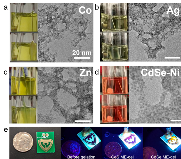
Figure 4. ME-gelation of MUA-capped CdS QDs using different metal anodes a-c, Co, Ag, and Zn, respectively, at 1.2 V and d, MUA-capped CdSe QDs using a Ni electrode. To the left of the TEM images are the corresponding photographs taken at 0 minutes (top) and 15 minutes (bottom) after the potential application. e, Photographs, from left to right: imaging under ambient light, a printed circuit board (PCB) chip patterned with an Au-coated electrode; imaging under ultraviolet light, the PCB chip after electrodeposition of Ni onto the electrode (before gelation), and after ME gelation of CdS, and CdSe QDs. A U.S. 10 cent coin (18 mm diameter) is included for scale.
