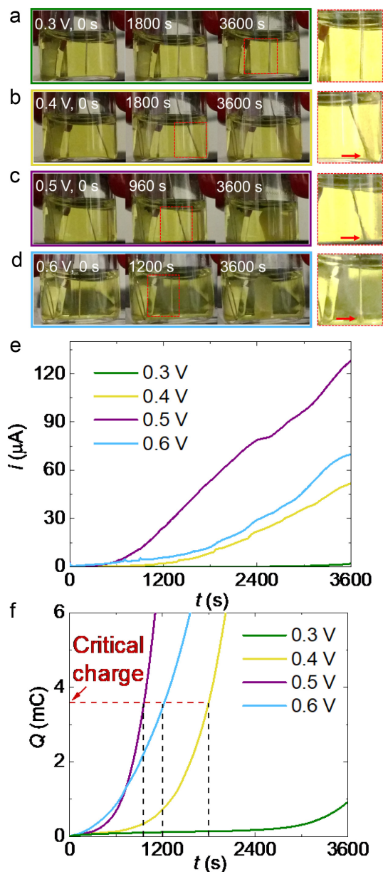
Figure 3. a-d, Photographs of CdS QD ME-gelation as a function of time at different applied electrode potentials from 0.3 V to 0.6 V vs Ag/AgCl/sat. KCl electrode. An expanded view of the working electrode at each gelation starting point is shown in the red-dashed box on the right. e and f, Current-time and charge-time traces for the corresponding ME-gelation potentials in a-d. Black dotted lines connect the observed gelation induction times to the charge-time traces.
