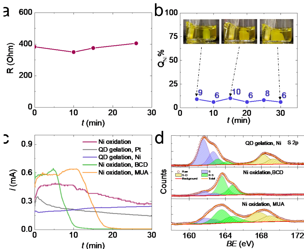
Figure 4. a Solution resistance ( R ) as a function of the electrogelation time ( t ) at 2 V. b Percentage charge used for Ni oxidation to \text{Ni}^{2+} during electrogelation ( Q_{\text{Ni}}\% ) at 2 V after 5 to 30 mins. c i - t traces for OE-gelation of CdS QDs at 2 V using a Pt electrode (gray line), Ni oxidation in methanol (containing 0.01 M TBAPF-6 but no QDs) at 2 V (red line), QD electrogelation using Ni at 2 V (purple line), and Ni oxidation at 2 V in a 5 mM BCD solution (green line) and 10 mM MUA solution (orange line). d XPS spectra of Ni electrodes used for QD electrogelation vs. oxidation in BCD or MUA solutions at 2 V.
