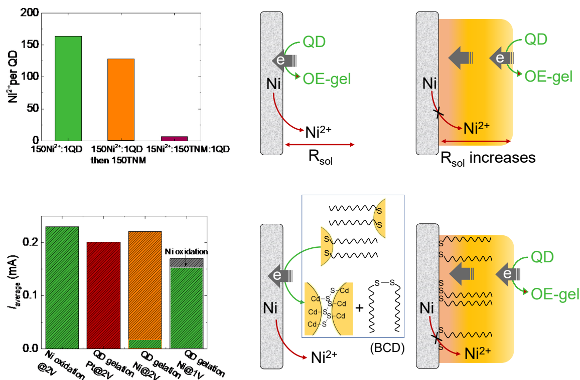
Figure 3. Electrogelation mechanism study. a The Ni 2+ /QD ratio in the QD gels prepared by mixing Ni 2+ and QDs at a molar ratio of 150: 1 (green bar), and with an additional 150 equivalents of chemical oxidant, tetranitromethane (TNM, orange bar), and with reduced equivalents of Ni 2+ (15Ni 2+ :150TNM:1 QD, red bar). b The average current ( i average ) for Ni oxidation in the absence of QDs at 2 V (green bar), QD electrogelation using a Pt electrode at 2 V (red bar), and QD electrogelation using a Ni electrode at 2 V (orange/green two-color bar) and 1 V (gray/green two-color bar). The green portion of the two-color bars represents the specific current for Ni oxidation obtained by analyzing the total amount of Ni 2+ released during electrogelation. c, d Two hypotheses that explain the suppressed Ni 2+ release during QD electrogelation at 2 V.
