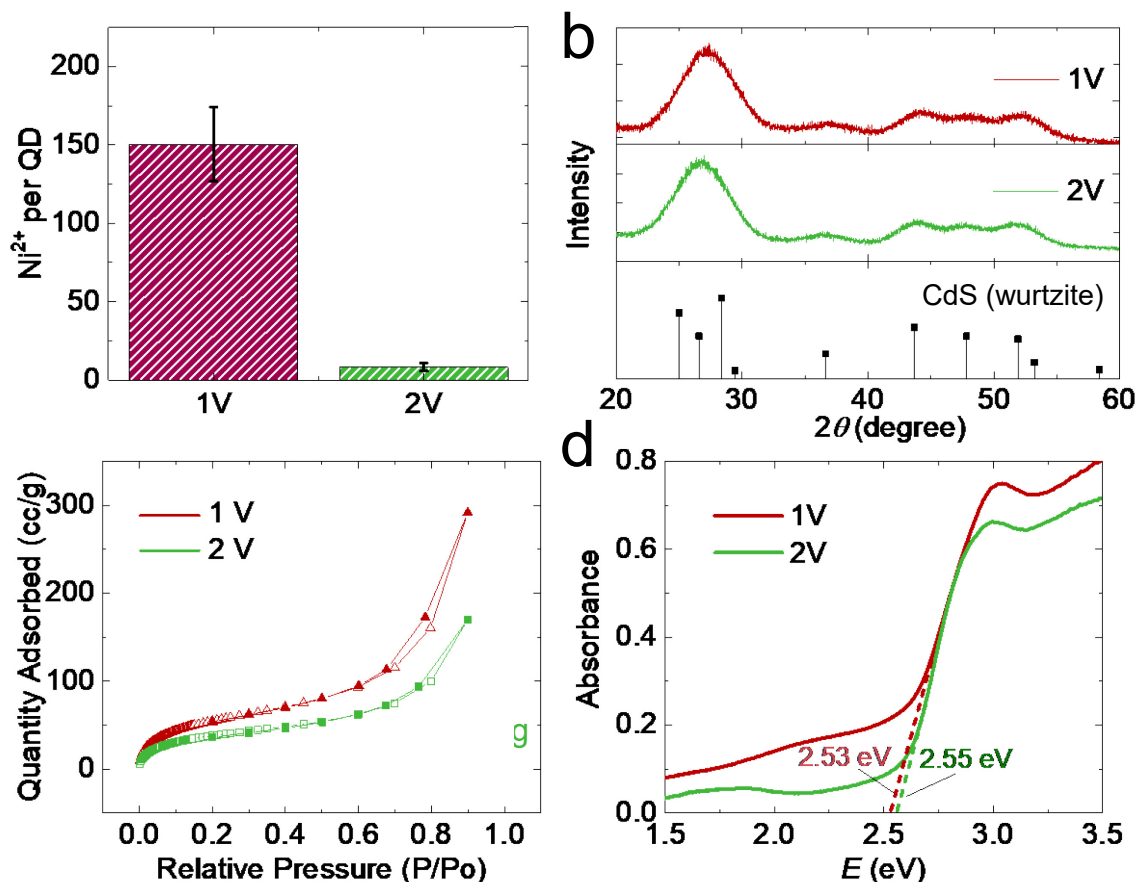
Figure 2. Compositional and structural characterization of QD electrogels synthesized at 1 V and 2 V. a \text{Ni}^{2+} /QD ratio in the gels. b Powder X-ray diffraction (PXRD) patterns. The stick diagram shows the PXRD pattern of hexagonal CdS (wurtzite) as a reference. c Nitrogen adsorption-desorption isotherms. d Solid-state diffuse reflectance data (converted to absorbance).
