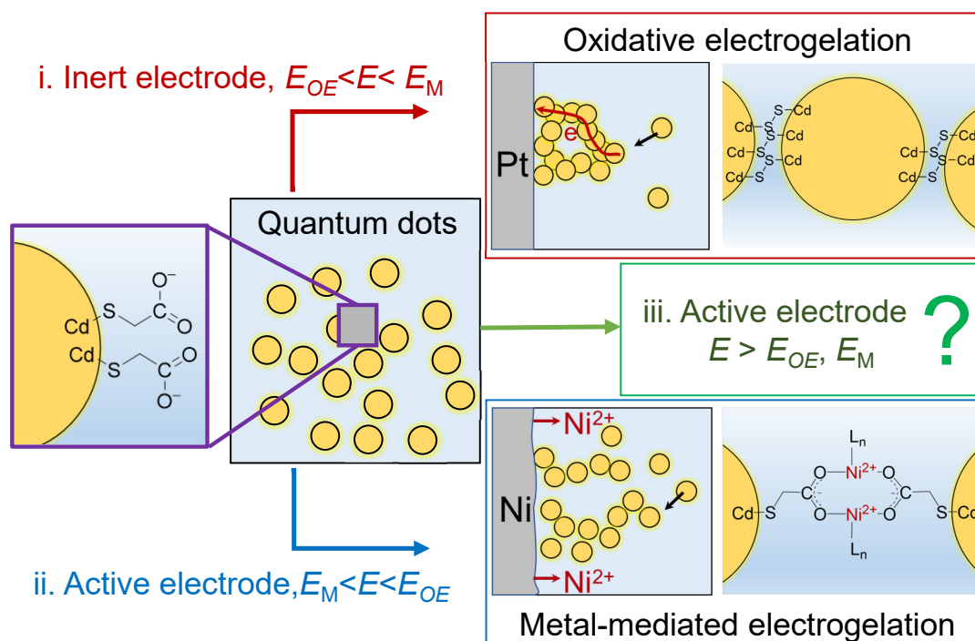
Scheme 1. Electrochemical gelation of metal chalcogenide QDs by different mechanisms. (i) Oxidative electrogelation (OE-gelation): the potential of an inert electrode (e.g., Pt) is sufficiently positive to oxidatively remove the thiolate ligands and form dichalcogenides bonds between QDs. (ii) Metal-mediated electrogelation (ME-gelation): an active electrode (e.g., Ni) undergoes electrodisolution due to its low oxidation potential, releasing metal ions to crosslink ligand-capped QDs bearing pendant carboxylates by forming coordination bonds between metal ions and QD-bound carboxylates. (iii) The focus of this study: the potential of an active electrode is positive enough to drive both OE- and ME-gelation. E : electrode potential; E_{OE} : the potential required for OE-gelation; and E_M : the electrode oxidation potential.
