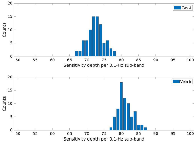
FIG. 5. Aggregated distributions of sensitivity depths (Eq. (11)) for Cas A (upper) and Vela Jr. (lower) based on 84 and 71 samples, respectively, of 0.1-Hz search sub-bands spanning the full 20–976 search band. The widths of the distributions are dominated by the depth variation with respect to frequency, which we empirically fit to a linear function of negative slope.
