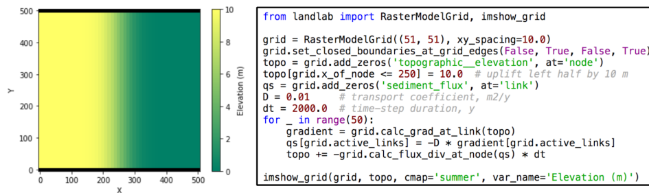
Figure 10. Example of a simple finite-volume numerical model of hillslope evolution, written in Python using the Landlab library. The model uses a diffusion equation to represent an evolving hillslope. The concise source code at right illustrates the use of a Landlab grid object together with fields and built-in functions for numerical gradient and divergence functions on these fields.
