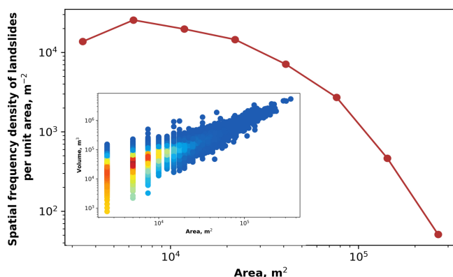
Figure 14. Magnitude–frequency relationship of the landslides simulated with Landlab-HyLands (red dots) and illustrated in Fig. 13. The inset shows a scatter density plot showing the simulated area–volume relationship.
