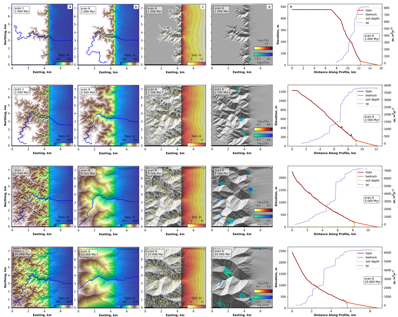
Figure 13. Illustration of HyLands model component. (a) Time slices showing evolution of the landscape to steady state without landsliding. The blue lines represent the plan-view locations of rivers plotted in the right-hand column. Column (b) is the same as column (a) but with landsliding. (c) Sediment accumulation and the formation of alluvial fans (with landsliding). (d) Landslide activity during the depicted time step. Red colors represent the logarithm of the landslide erosion depth; blue colors represent deposition. Column (e) shows the topographic and bedrock elevation (red and black line, respectively) and the sediment thickness (orange line). The sediment flux is plotted against the right-hand y axis (blue line). Note that during landsliding both pure landslide dams (red bumps on the profile) and irregularities in the bedrock profile (grey bumps) arise. The latter originate from the river being redirected after landsliding, forming epigenetic gorges.
