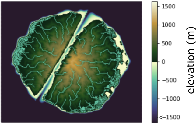
Figure 12. Snapshot of prototype integrated numerical model of landscape and sedimentary basin evolution. Domain size is 250 by 250 km. Simulation shows a hypothetical micro-continent with an active NNE-oriented extensional fault. Sea level varies stochastically; this particular snapshot captures a period of rising sea level after a brief low stand. Model was constructed using Landlab components for flow routing (FlowAccumulator, FlowDirectorSteepest, LakeMapperBarnes), fluvial processes (ErosionDeposition), marine sediment transport (SimpleSubmarineDiffuser), lithosphere flexure in response to loading and unloading (Flexure), and extensional faulting (ListricKinematicExtender). Color map designed by Thyng et al. (2016).
