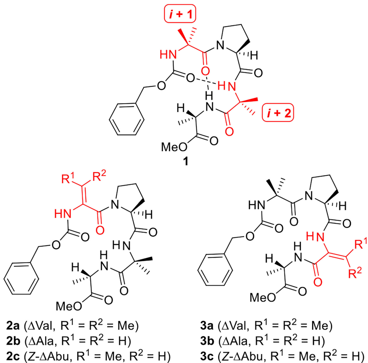
Figure 2. Balaram's incipient 3_{10} helical peptide (1) and proposed \Delta AA-containing variants (2 and 3).
