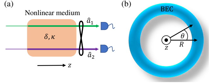
FIG. 3. Experimental implementations. (a) Schematic optical setup for realizing pseudo- \mathcal{APT} -symmetry physics through nonlinear spontaneous four-wave mixing. (b) Experimental realization based on a cold atomic BEC in a ring trap.
