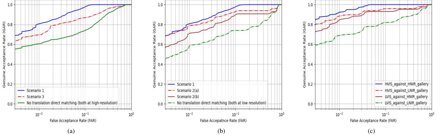
Fig. 5. ROC plots showing the performance of our approach (a) Scenario 1 and 3 with cGAN architecture, (b) Scenario 2(a) and 2(b) with cGAN architecture and (c) cpGAN architecture obtained on the PolyU Bi-Spectral database for the different cross-spectral matching scenarios [17].
