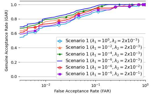
Fig. 11. Comparative ROC results showing the sensitivity of matching performance on the hyperparameters of our proposed cGAN, when it is trained only on the PolyU Bi-Spectral dataset for Scenario 1.
