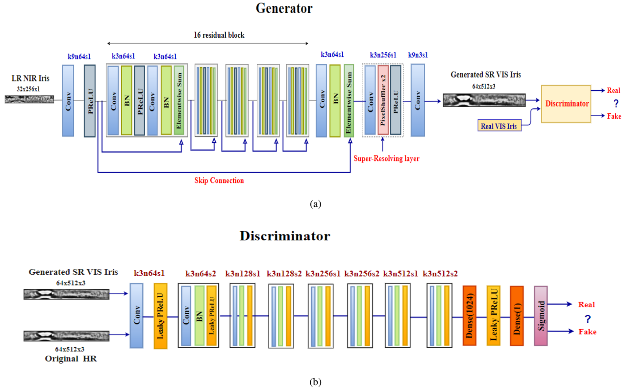
Fig. 4. Architecture of our proposed cGAN (a) generator and (b) discriminator with corresponding kernel size (k), number of feature maps (n) and stride (s) indicated for each convolutional layer.
