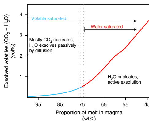
Fig. 2 | Plot depicting the increase in the volume of exsolved volatiles (CO 2 + H 2 O) with crystallization. The calculations are made for storage of a rhyolitic magma at a pressure of 2 kbar. The exsolution is modelled using rhyolite-MELTS 40 , starting from the composition of the Nikiya lava flow from Nisyros volcano 35 , with an initial 4.5 wt% of dissolved H 2 O and 500 ppm CO 2 , as it cools from 950 °C to 730 °C. Blue indicates the increase in exsolved volatiles during water-undersaturated differentiation, while red depicts the same for water-saturated crystallization. The dashed lines mark the moment of water saturation.
