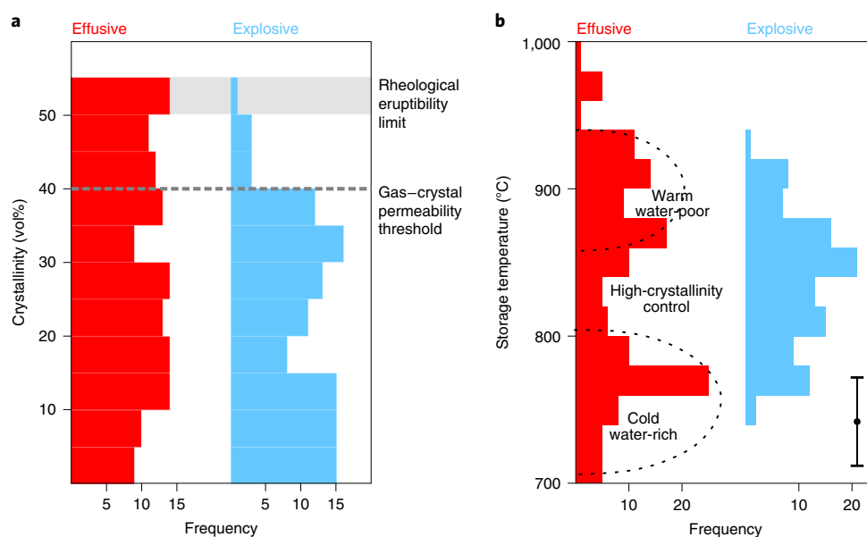
Fig. 4 | The distribution of crystallinity and storage temperatures with eruptive behaviours. a, b , Histograms showing the distribution of crystallinity ( a ) and storage temperatures ( b ) with eruptive behaviours. The frequency of explosive events decreases drastically at crystallinities >40 vol% (horizontal dashed grey line in a ), while effusive events occur over the entire crystallinity range (0–55 vol%). Magmas behaving explosively seem to be stored in a relatively well-constrained interval of temperatures, roughly between 770 and 900 °C with a maximum frequency between 800 and 880 °C. Effusive events occur over a larger interval of storage temperatures (700–1,000 °C), with maximum frequency at <800 °C (colder temperatures characteristic of differentiated magmas at water saturation) and >850 °C (warmer temperatures favouring lower melt viscosities and gas permeability development 24 ) (areas enclosed by black dashed lines in b ).
