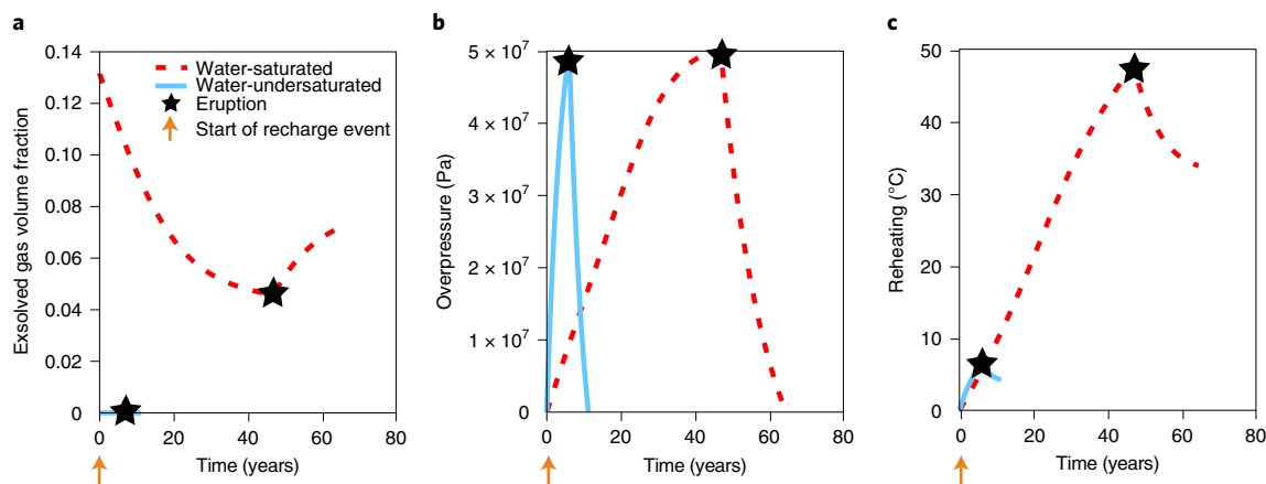
Fig. 5 | Response of reservoirs containing water-saturated and water-undersaturated magmas to recharge events. The results are derived from running a new simulation with a published numerical model 34,56 for the typical case of effusive and explosive eruptions at Nisyros volcano. The maximum overpressure required to initiate an eruption is set to 50 MPa. The size of the reservoir (30 km 3 ), the temperature of recharge (950 °C) and the recharge rate over time (0.1 km 3 yr -1 ) are the same between the two examples and are kept constant. The water-undersaturated magma has a pre-recharge storage temperature of 820 °C, while the water-saturated magma has a colder storage temperature of 750 °C and an initial volume of exsolved gas >10%. a , The decrease in the volume fraction of exsolved gas in response to the influx of mafic recharge, caused by the compressibility of the exsolved gas and, to some degree, by re-dissolution due to pressure increase. b , All else being equal, the existence of a compressible exsolved volatile phase requires a greater amount of mass injected in the chamber to reach the critical overpressure that initiates the eruption. At a constant recharge rate, this translates into longer recharge times. c , The compressibility–reheating feedback, with the water-saturated reservoir being subjected to greater volumes of hot recharge over a longer time period, resulting in a greater temperature increase.
