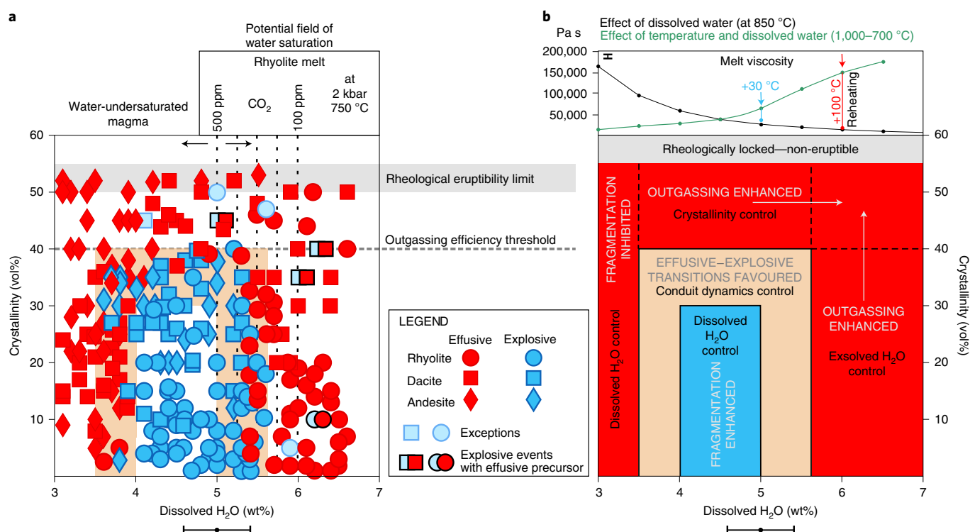
Fig. 3 | Correlation of eruptive styles with crystallinity, dissolved H 2 O and water saturation. a, b. The data (a) and the results translated into a regime diagram (b). The potential field of water saturation is calculated for a magma with rhyolitic melt stored at 2 kbar (ref. 44 ). For illustrative purposes, we use a temperature of 750 °C and varying CO 2 concentrations (vertical dashed lines in a). The data show a clear window of explosivity separated from the effusive domain by a transitional field (orange background). In the transitional field, water content and crystallinity fail to discriminate between effusive and explosive eruptions. According to the data, this corresponds to magmatic conditions at which both eruptive styles are possible and the ensuing eruptive behaviour is likely to be dominantly controlled by the conduit dynamics. Outside this field, the magmatic properties inherited from the magma chamber predetermine the eruptive behaviour. The crystallinity threshold at which permeable outgassing is favoured 51 and the rheological eruptibility limit 59 are also depicted. Above the regime diagram, the evolution of melt viscosity 54 with (1) increasing dissolved water at constant temperature (black curve, 850 °C) and (2) the combined effect of increasing dissolved water and magmatic cooling (green curve) is depicted. For the viscosity calculation, the thermal and water-content evolution is modelled using rhyolite-MELTS 40 , starting from a dacitic composition at 3 wt% dissolved water over a cooling range from 1,000–700 °C. The water-undersaturated and saturated melts are reheated by 30 °C (at 5 wt% H 2 O) and 100 °C (at 6 wt% H 2 O) to test the effect that hot recharge has upon eruptive melt viscosity for a Nisyros-type explosive (blue line) and effusive case (red line) 35 . For the uncertainty calculation on dissolved H 2 O, we use the average relative errors of the storage temperature and the uncertainty of the hygrometer, which we propagate in quadrature. The average propagated error of the dissolved water content over the interval analysed is 9.2% relative, which translates to the average absolute error of ±0.41 wt% H 2 O.
