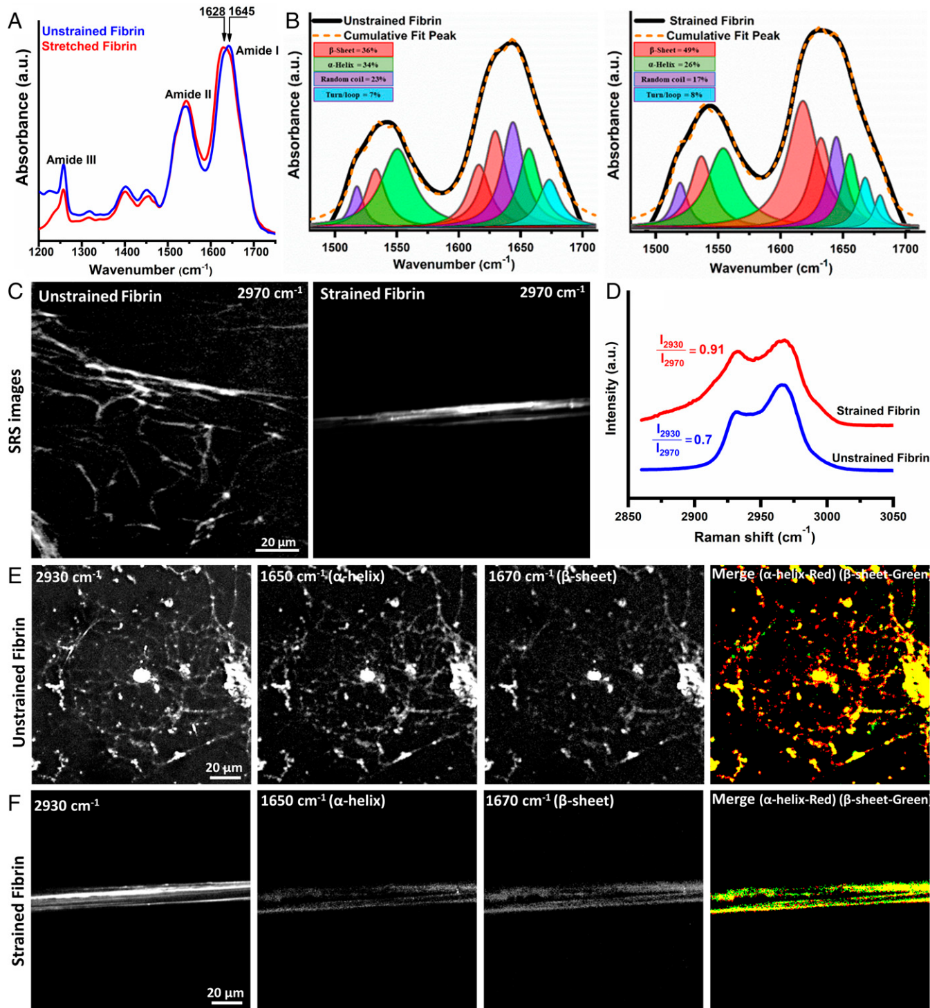
Fig. 2. Tensile strain causes fibrin molecular and structural unfolding. (A) ATR-IR spectra of unstrained and 100% strained fibrin showing amide I to III bands with a clear amide I peak shift showing structural changes. (B) Decomposition of amide I and II modes from spectra in (A) into constituent peaks corresponding to different protein secondary structures shows the increased \beta -sheet content with strain. (C) SRS CH stretch (2,970 cm -1 ) image, (D) CH stretch spectra from 2,850 to 3,050 cm -1 of unstrained and strained fibrin. (E) and (F) SRS images from strained and unstrained fibrin acquired at the CH 3 mode (2,930 cm -1 ), \alpha -helix mode (1,650 cm -1 ), \beta -sheet mode (1,670 cm -1 ), and thresholded overlapped \alpha -helix (red) and \beta -sheet (green) images. Imaging conditions were identical for all SRS images at the respective wavenumbers.
