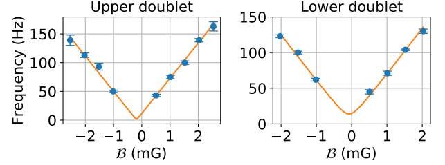
FIG. 5. Energy differences between the m_F = \pm 3/2 states; measurement of the magnetic g -factors. The fits are performed with our model which takes into account the avoided crossing introduced by going into the rotating frame of the molecules. The energy difference at the avoided crossing is fixed by our ab initio calculations. The only fit parameters are the asymptotic gradients (corresponding to 3g_{F=3/2}\mu_B/h ) and the horizontal offset due to ambient fields. The error bars are 1\sigma error estimates extracted from a non-linear fit to each Ramsey fringe.
