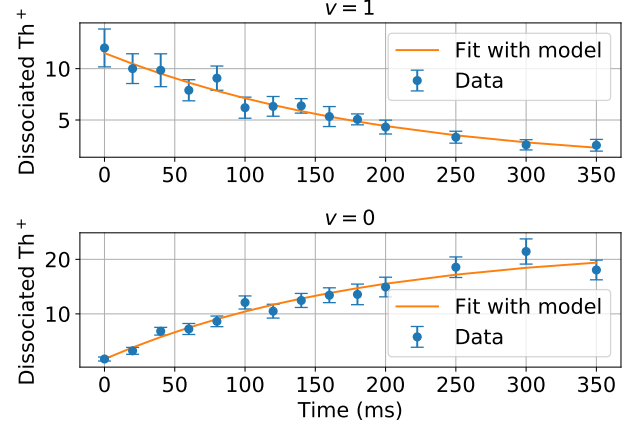
FIG. 8. Vibrational population decay from v=1 to v=0 of the ground electronic state in \text{ThF}^+ . All the population was pumped from the ground vibrational manifold into the excited vibrational manifold through the \Omega = 0^- state [26]. Population in each vibrational manifold is read out with photodissociation. The observed vibrational decay lifetime agrees with our model, which is used to predict the blackbody radiation excitation lifetime from X^3\Delta_1 . The total dissociated \text{Th}^+ numbers do not appear to be conserved in these two plots because the dissociation efficiencies for these two vibrational manifolds are not the same.
