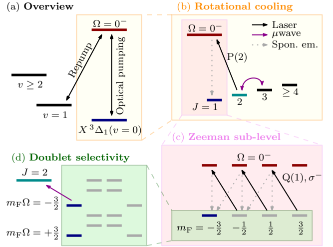
FIG. 1. State preparation sequence (not to scale). (a) All our optical pumping lasers connect from the X^3\Delta_1(v=0) vibronic manifold to the \Omega=0^- ( v=0 ) vibrational manifold [26]. We have a vibrational repump laser from the X^3\Delta_1(v=1) manifold. (b) Within the X^3\Delta_1(v=0) vibronic manifold, we perform rotational cooling by optically pumping the J=2 state through the \Omega=0^- state. We use microwaves to couple the J=2 and J=3 states together to transfer J=3 population eventually into J=1 . (c) Within the J=1 manifold, we pump all the ions into a single Zeeman m_F state using circularly polarized light on the Q(1), \sigma^- line. We also introduce a magnetic field to prevent the Zeeman levels from mixing through rotation coupling (refer to Section II C). (d) \Omega -doubling gives rise to two closely spaced states with the same m_F number. We can deplete one of these states by coupling it with microwaves to J=2 . The state preparation process is shown as a sequence of steps for clarity, but all the steps involved occur at the same time in our experiment.
