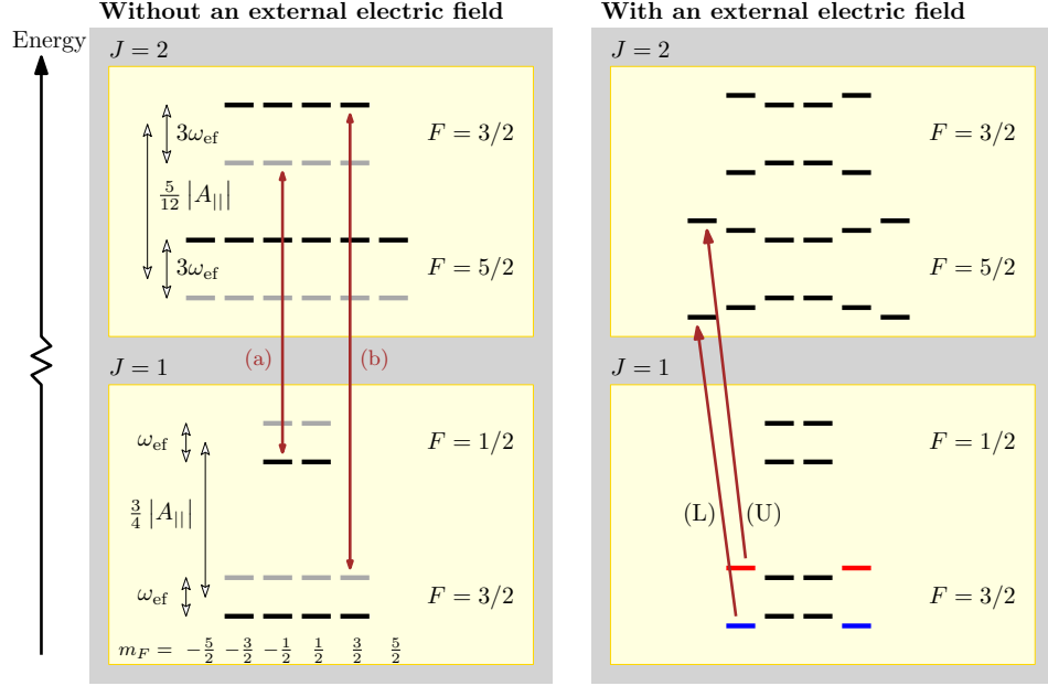
FIG. 2. Energy landscape (not to scale) of the neighborhood of the eEDM-sensitive state X^3\Delta_1(v=0) , showing only the first two rotational levels. In the absence of external electric field, the eigenstates are states of good parity. The energy levels with positive (negative) parity are denoted by black (grey) lines in the energy level diagram on the left. Selection rules for E1 transitions only allow for transitions connecting states of opposite parities, \Delta F = 0, \pm 1 , and \Delta m_F = 0, \pm 1 , thus resulting in only six distinct frequencies for resonant transitions connecting the J = 1 to J = 2 rotational manifold in the absence of an external magnetic field. For example, the transitions with the highest and lowest frequencies are labelled (a) and (b), respectively, here and also in Figure 3. In the presence of an external electric field, states of opposite parities mix. The red arrows on the right panel labeled (L) and (U) correspond to the stretched-to-stretched transitions used to determine the Stark shift in our microwave spectroscopy. The Stark shift depends on m_F and d_{mf} . The eEDM-sensitive states used for the eEDM measurement are the upper (red) and lower (blue) doublets. To reduce clutter in the diagrams, the states drawn do not reflect the true nature of the states in three aspects: (i) the states are drawn with an artificially large A_{||} in comparison to \omega_{ef} for well separated hyperfine levels in the diagram; (ii) the Stark shifts in the diagram are portrayed proportionally smaller than those in the actual experiment, where Stark shifts are large enough to allow some states in the lower hyperfine level to be more energetic than the upper; and (iii) F is no longer a good quantum number in the presence of a strong external electric field, except for the most stretched Zeeman states in each rotational manifold. Hence, in the presence of an external electric field, the only selection rule remaining on the J = 1 to J = 2 transition is \Delta m_F = 0, \pm 1 .
