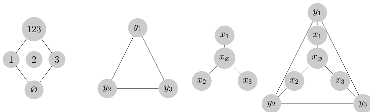
Figure 1: The poset \mathcal{F}(M) and the complexes \mathcal{I}(M) , \mathrm{Cone}(\underline{\Delta}_M) , and \Delta_M from Example 4.
