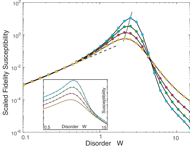
FIG. 1. Typical scaled fidelity susceptibility \exp[\zeta]/2^L (main plot) and the unscaled one \exp[\zeta] (inset) as a function of disorder W for different system sizes L = 12, 14, 16, 18 (yellow to blue). The dashed line shows the ETH prediction. The dotted line shows the predicted peak drift with the system size: \chi_{\max} = c \exp[\alpha W^*] , where W^* = L \log(2)/\alpha [see Eq. (11)]. Yellow, green, and blue shaded regions correspond to ergodic, glassy, and localized phases. As the system size increases, the green blue crossover boundary drifts to stronger disorder values.
