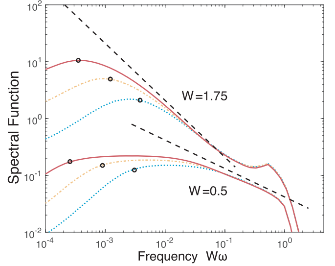
FIG. 3. Spectral function II. The Fourier transform of the infinite temperature connected two-point correlation of the local z magnetization is shown for two values of the disorder, W = 0.5 and W = 1.75 , for chains of size L = 12, 14, 16 in blue dots, yellow dash-dot, and full red, respectively. Heisenberg time is indicated by the black circles. The black dashed lines show 1/\sqrt{\omega} and 1/\omega asymptotes.
