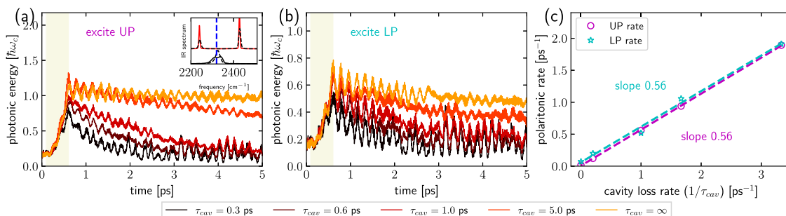
FIG. 3. The same plot as Fig. 2 when the CO 2 molecular density is decreased from 1.101 to 0.073 g/cm 3 and all other simulation details are kept the same. In the inset of (a), the black dashed lines represent the corresponding spectra in Fig. 2 and the solid lines represent the spectra when the density is reduced. As shown in the inset, the Rabi splitting is largely unchanged when the molecular density changes.
