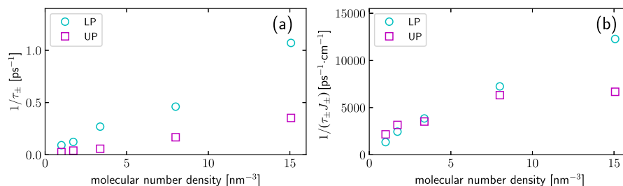
FIG. 5. (a) Polariton decay rate ( 1/\tau_{\pm} ) vs the molecular number density when \omega_c = 2320 \text{ cm}^{-1} and \tilde{\epsilon} = 2 \times 10^{-4} a.u. Here, the molecular density is changed by tuning the simulation cell length while keeping the molecular number the same (so the Rabi splitting is fixed). See Sec. II B 1 for other simulation details. (b) The corresponding 1/(\tau_{\pm}J_{\pm}) vs the molecular number density.
