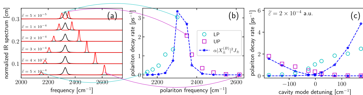
FIG. 4. Polariton decay rate vs Rabi splitting and cavity mode detuning. (a) Simulated IR spectrum for liquid CO 2 inside (red lines) or outside (black lines) a cavity. The cavity mode frequency ( \omega_c ) is set as 2320 cm -1 . From top to bottom, the effective coupling strength is labeled on each line shape (from 5 \times 10^{-5} to 5 \times 10^{-4} a.u.), respectively. (b) Simulated polariton decay rate for the polaritons in (a) (cyan circles for the LP and magenta squares for the UP, the same as below). Blue stars plot \alpha|X_{\pm}^{(B)}|^2 J_{\pm} , where |X_{\pm}^{(B)}|^2 J_{\pm} is defined in Eq. (23) and \alpha = 1200 ps -1 /cm is a prefactor to best fit the polaritonic decay rates. (c) Polariton decay rate and the corresponding \alpha|X_{\pm}^{(B)}|^2 J_{\pm} vs the cavity mode detuning ( \omega_c - \omega_0 ) when \tilde{\epsilon} = 2 \times 10^{-4} a.u., where \alpha takes the same value as that in (b). See Sec. II B 1 for other simulation details.
