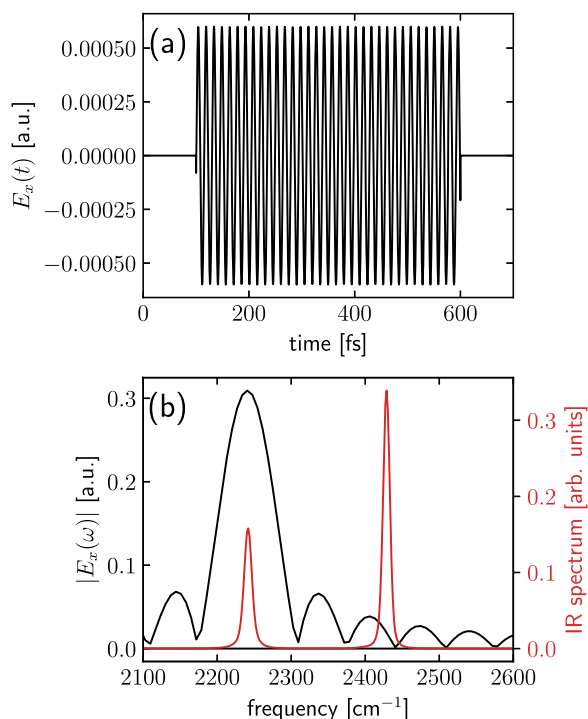
FIG. 6. (a) The E-field profile E_x(t) defined in Eq. (21), where the pulse frequency is set as the LP frequency of Fig. 2: \omega = \omega_{LP} = 2241 \text{ cm}^{-1} . (b) The corresponding E-field spectrum in the frequency domain. The red line replots the Rabi splitting spectrum in the inset of Fig. 2(a).
