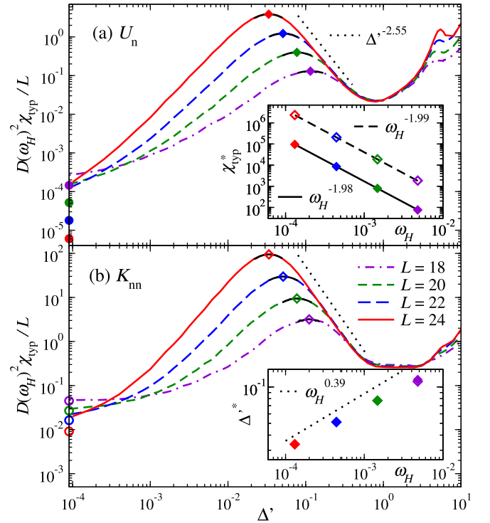
FIG. 1. Typical fidelity susceptibility \chi_{\text{typ}} (scaled to exhibit collapse in the quantum-chaotic regime) vs the integrability-breaking parameter \Delta' for observables \hat{U}_{\text{n}} (a) and \hat{K}_{\text{nn}} (b) in clean periodic chains. To calculate \chi_{\text{typ}} and \omega_H , we average over the central 50% of the eigenstates in the even- Z_2 sector in each total quasimomentum sector considered. For L < 24 , we report the weighted average over all k \neq (0, \pi) sectors, while for L = 24 we report results for the k = \pi/2 sector. Circles on the y axis show \chi_{\text{typ}} at the integrable point ( \Delta' = 0 ), and diamonds show the maximal \chi_{\text{typ}}^* (at \Delta'^* = -b/2a ) obtained from polynomial fits ax^2 + bx + c (black solid lines about the maxima). The dotted lines on the right of the first peaks are a guide for the eye and depict \Delta'^{-2.55} behavior. Inset in (a): \chi_{\text{typ}}^* vs \omega_H for both observables, along with the results of power-law fits. Inset in (b): \Delta'^* vs \omega_H for both observables (the values of \Delta'^* overlap). The dotted line depicts \omega_H^{0.39} behavior.
