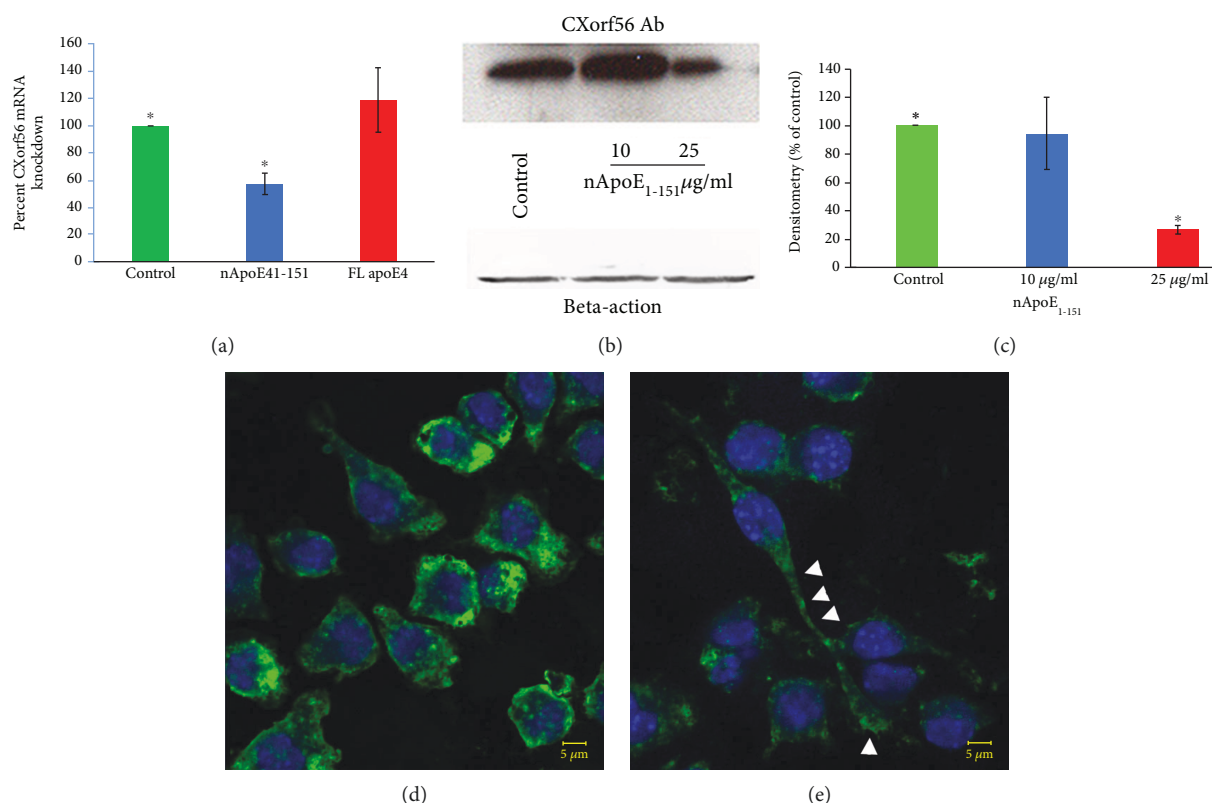
FIGURE 5: Treatment of BV2 microglial cells with an amino-terminal fragment of apoE4 leads to the downregulation of CXorf56. (a) BV2 cells were treated for 5 hours with 25 μg/mg nApoE4 1-151 (blue bar) or with an equivalent concentration of full-length apoE4 (red bar). Following treatment, RNA was extracted and RT qPCR was performed. Data indicated a significant decrease in the expression of the CXorf56 homologue following treatment, p = 0.0002 , while full-length apoE4 had no significant effect. (b, c) Western blot analysis utilizing an anti-CXorf56 antibody (1:500) confirmed the decreased expression of the CXorf56 protein following treatment of BV2 cells for 24 hrs with 25 μg/ml nApoE4 1-151 . Beta-actin was employed as a loading control utilizing an anti-beta-actin antibody (1:50K), bottom panel. (c) Quantitative densitometry analysis of 3 independent experiments showing an overall 74% decrease in the expression of CXorf56 protein following treatment (* denotes p = 5.76 \times 10^{-7} ). Data are representative of 3 independent experiments \pm S.D. (d, e) BV2 cells were left untreated (d) or treated for 24 hours with nApoE4 1-151 and stained with the CXorf56 antibody. Following treatment, there was a decrease in the staining intensity as well as a morphological shift to bipolar, extended pseudopods (arrowheads, e).
