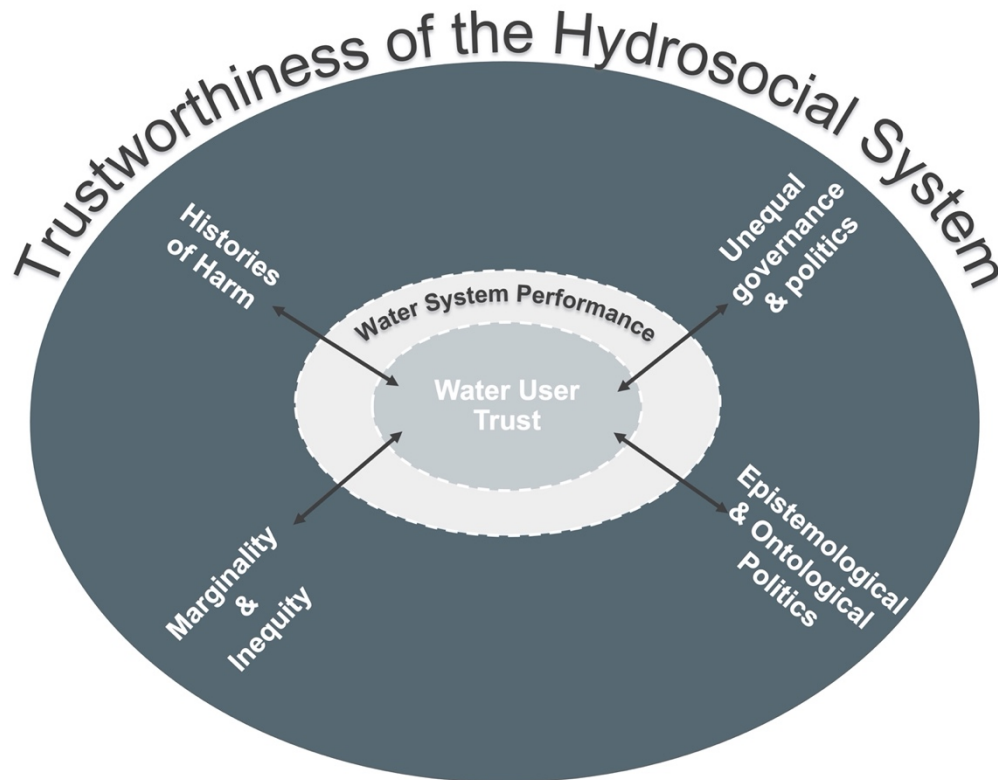
Figure 1 Conceptual diagram illustrates the need to move from a focus on individual trust to examine the trustworthiness of the broader hydro-social system as shaped by water system performance and interconnected factors including experiences of marginality and inequity, ontological and epistemological injustice, unequal governance and politics, and histories of water insecurity and harm.
