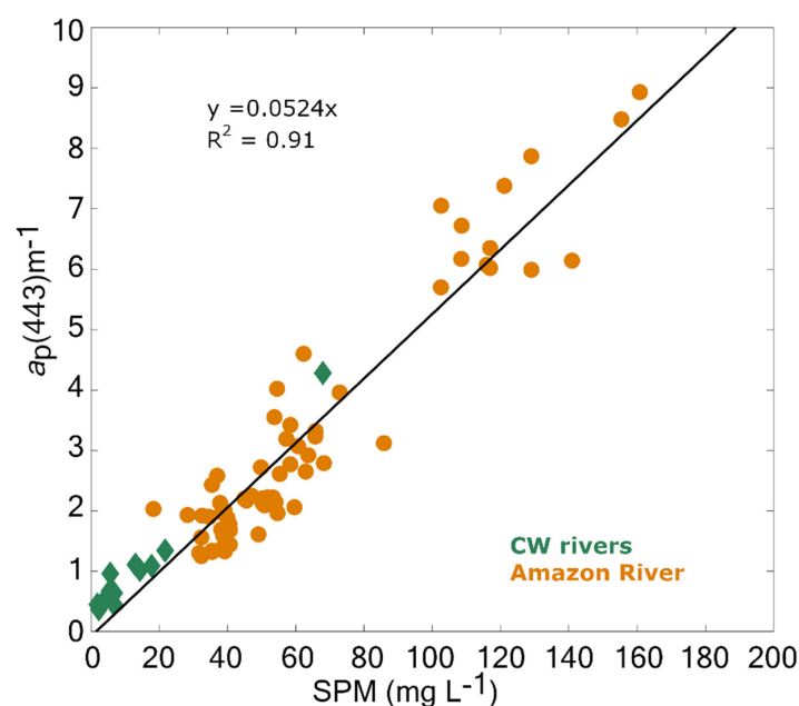
Figure 3. Scatterplot of a_p(443) as a function of suspended particulate matter. A linear regression with null intercept is shown by the solid black line.
