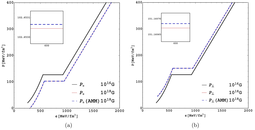
Fig. 3. (Color online) Parallel (a) and perpendicular (b) EOS in the Maxwell construction including (blue-dashed) the neutron AMM at B^{\text{HP}} = 10^{18} G and excluding the neutron AMM at B^{\text{HP}} = 10^{18} G (red-dotted) and at B^{\text{HP}} = 10^{16} G (black-solid).
