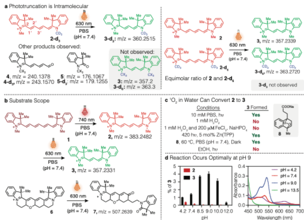
Figure 2. Mechanistic studies of cyanine phototruncation. (a) Products observed following irradiation of 2-d 3 or an equimolar ratio of 2 and 2-d 6 in PBS (100 \mu M, 1 mL, with 0.01% DMSO, pH = 7.4) with 630 nm LED at 0.2 W cm -2 for 60 minutes and monitored by HRESIMS. (b)
