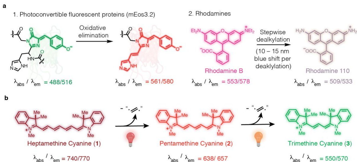
Figure 1. Key background and current studies. (a) Photoconversion reactions in common fluorophores. (b) Cyanine phototruncation reaction reported here. Wavelengths in nm.
