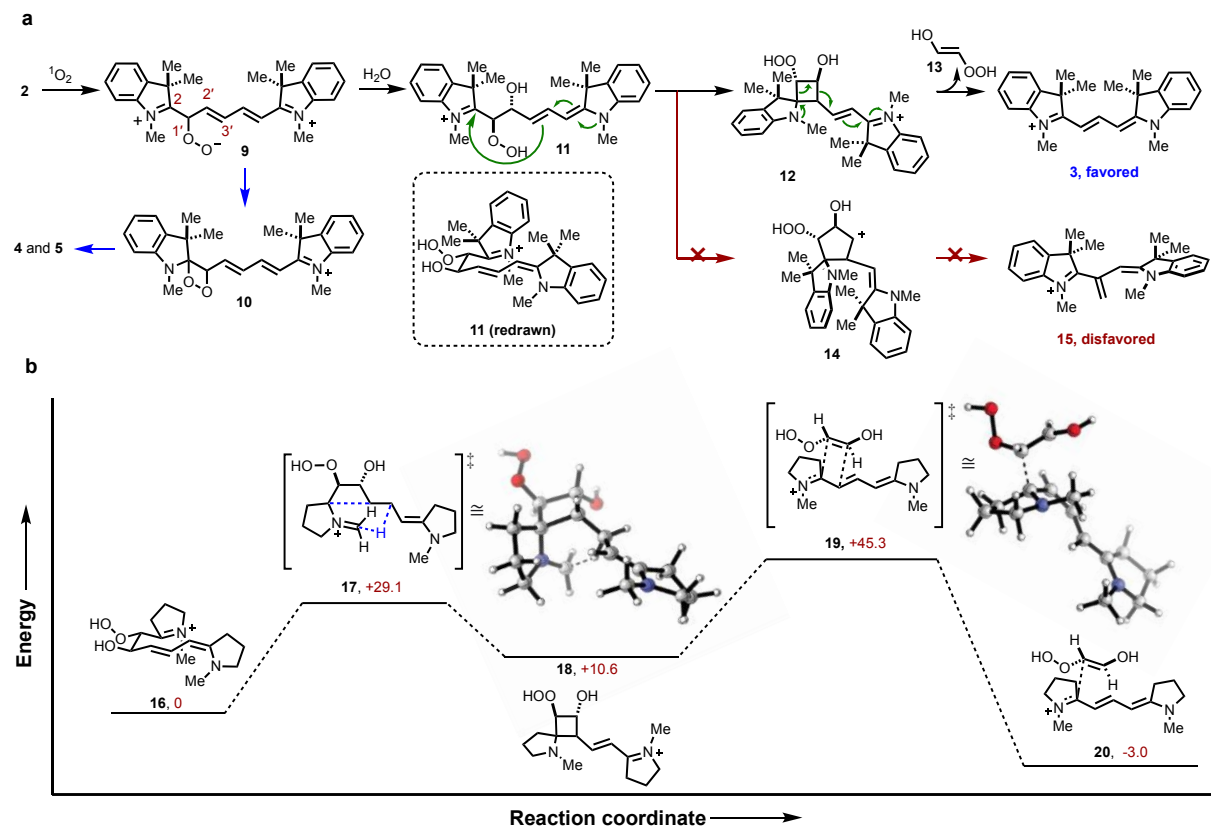
Figure 3. Mechanistic proposal and computational analysis. (a) Proposed mechanism of cyanine phototruncation with the representative conversion of 2 to 3 . (b) DFT computed potential energy surface for conversion of 16 to 20 . Computed surfaces showing the results of ground state DFT calculations using M062-X/6-31G(d,p). Relative enthalpies ( \Delta H ) are given in kcal/mol.
