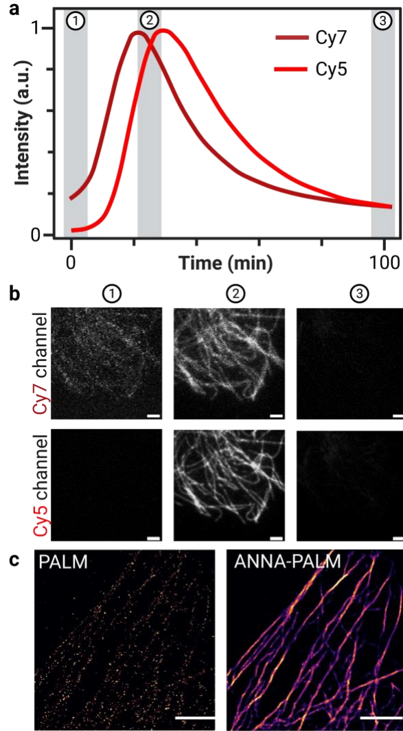
Figure 5. Cyanine phototruncation enables SMLM. TIRF-imaging of IgG-gar-Cy7 (DOL \sim 4 ) immunolabeled microtubules in COS7 cells using solely 640 nm irradiation. (a) Time course of fluorescence signals recorded on a longer wavelength Cy7 channel and a shorter wavelength Cy5 channel. (b) Fluorescence imaging was performed in 1 M CAPSO, pH 9.5 at the designated time points (1-3) using an irradiation intensity of 0.1 \text{ kW cm}^{-2} . Band pass filters used: Cy5 red-channel (679/41 nm) and Cy7 far-red channel (835/35 nm). (c) SMLM image of microtubules reconstructed after an acquisition time of 83.3 min at 100 ms exposure time using solely 640 nm irradiation at an intensity of 0.5 \text{ kW cm}^{-2} . The left image shows the raw reconstructed PALM-like, i.e., Cy5 is photoactivated via phototruncation \text{Cy7} \rightarrow \text{Cy5} followed by detection, localization, and photobleaching or further photoconversion. SMLM image obtained after applying a trained artificial neural network (ANNA-PALM) algorithm 15 to the reconstructed raw PALM image. Scale bars: 2 \mu\text{m} (b,c).
