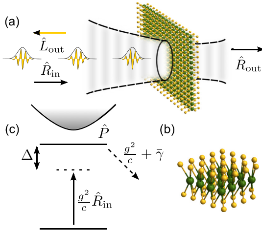
FIG. 1. (a) A quantum light field \hat{R}_{\text{in}} impinges on a two-dimensional semiconductor. Under strong driving, its largest fraction is transmitted into \hat{R}_{\text{out}} , while well-separated photons are back-reflected into \hat{L}_{\text{out}} . (b) Atomistic model of a monolayered transition metal dichalcogenide, where a layer of transition metal atoms (green) is sandwiched between chalcogen atoms (yellow). (c) The exciton resonance is described by bosonic operators \hat{P}(\mathbf{r}) , coupled to the laser field at a coupling strength g with a detuning \Delta . This coupling produces a natural decay rate \gamma = g^2/c , which can be elevated by additional decay and dephasing \bar{\gamma} .
