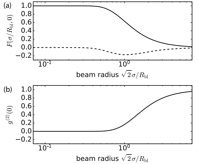
FIG. 2. Reflection properties for various beam sizes. (a) Nonlinear reflection, as characterized by the dimensionless function F , reaches a maximal plateau value when \sigma < R_{bl} and falls off for larger beam radii, shown in terms of the function F defined in Eq. (23) for resonant driving ( \varphi = 0 ). The solid line represents the real part (nonlinear reflection), the dashed line represents the imaginary part (nonlinear refraction). (b) The equal-time correlation function g^{(2)} of reflected light is strongly suppressed for small beams radii.
