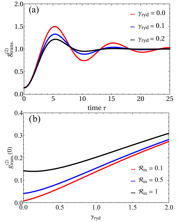
FIG. 7. Effects of Rydberg decay \gamma_{\text{ryd}} on light correlations. (a) Examples of the correlation function for different \gamma_{\text{ryd}} at \mathcal{R}_{\text{in}} = 1 and \Omega = 0.3 . (b) Zero-time antibunching in the transmitted photons tends to decrease with \gamma_{\text{ryd}} and \mathcal{R}_{\text{in}} but remains at remarkably high levels even in the presence of large Rydberg decay.
