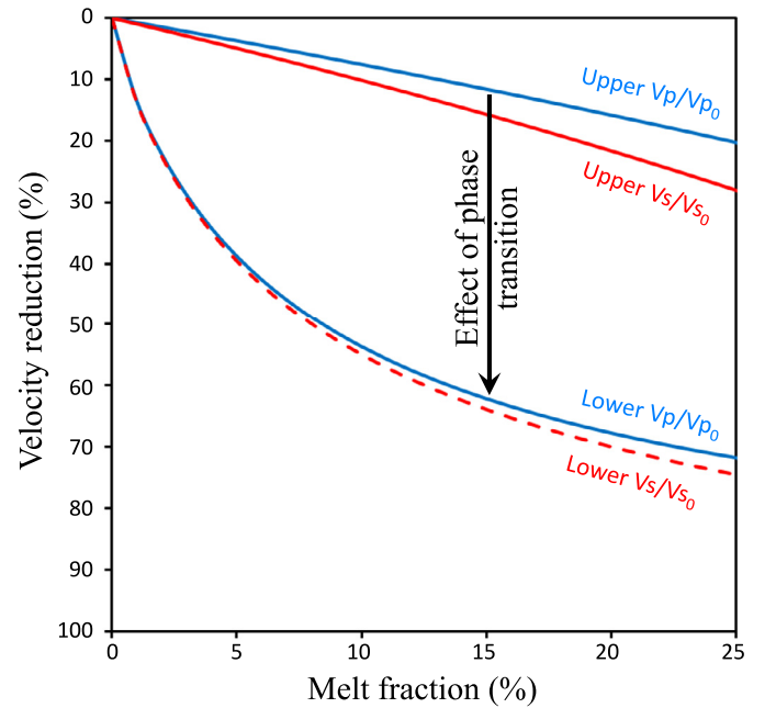
Fig. 7. Velocity change predicted by the model with spherical inclusions and corrected after the phase transition effect for S_0 = 5.0 mm, a = 5 MPa/°K, and 1 Hz frequency.
