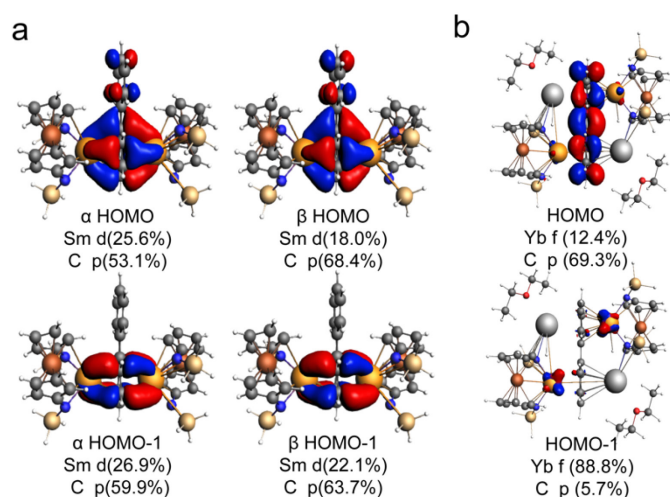
Figure 4. Kohn-Sham representations of HOMO and HOMO-1 and main atomic orbital contributions for (\text{Sm}_2\text{-biph})^{2-} (a) and \text{Yb}_2\text{-biph-K}_2 (b). The alkyl substituents on the silicon atoms were replaced by hydrogen atoms for simplification (iso = 0.03).
