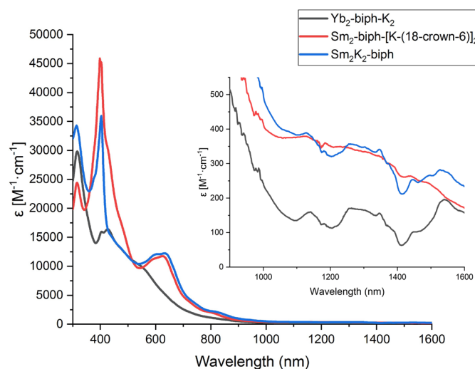
Figure 3. UV/Vis/NIR spectra of Yb 2 -biph-K 2 (black), Sm 2 -biph-[K(18-crown-6)] 2 (red), and Sm 2 -K 2 -biph (blue) in THF at room temperature. The NIR region from 1000–1600 nm is enlarged in the upper right corner.
