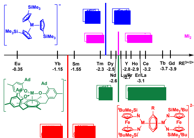
Chart 1. Scale of M^{3+/2+} ( M = rare earth metal) reduction potentials 28 and electron configurations of divalent rare earth metal complexes in different coordination environment: pink, M(II)I_2 ; 29 blue, [K(crypt)](Cp_3M) ; 39 green, [K(crypt)](((Ad,Me)ArO)_3mes)M ; 42 red, [(NN^{TBS})M]_2(\mu-biphenyl)[K(solvent)]_2 (this work).
