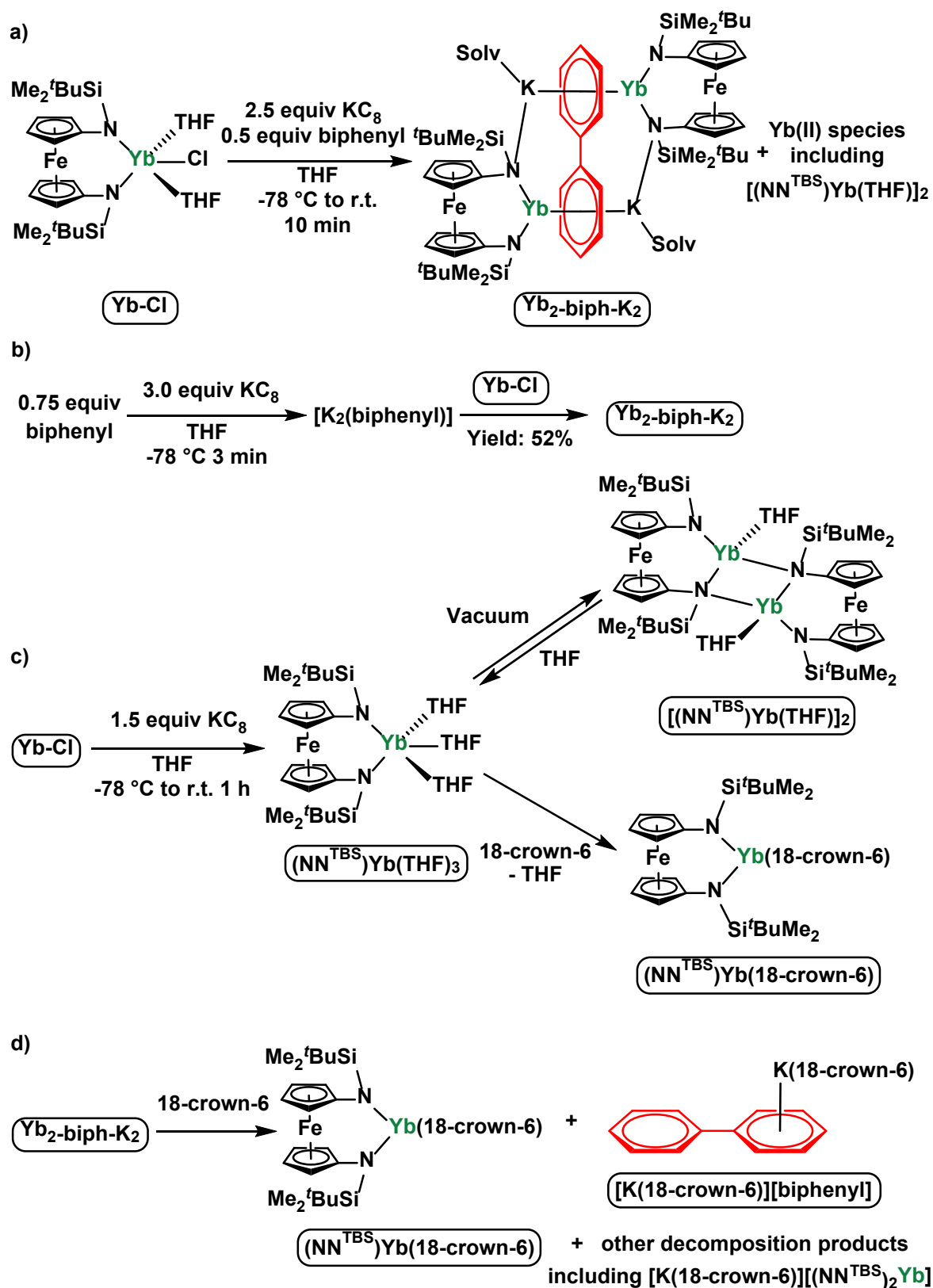
Scheme 2. (a) One-pot reduction of Yb-Cl and biphenyl by KC 8 ; (b) Optimized synthesis of Yb 2 -biph-K 2 by pre-mixing an excess of biphenyl and KC 8 ; (c) Direct reduction of Yb-Cl and transformations of Yb(II) products; (d) Reaction of Yb 2 -biph-K 2 with an excess of 18-crown-6.
