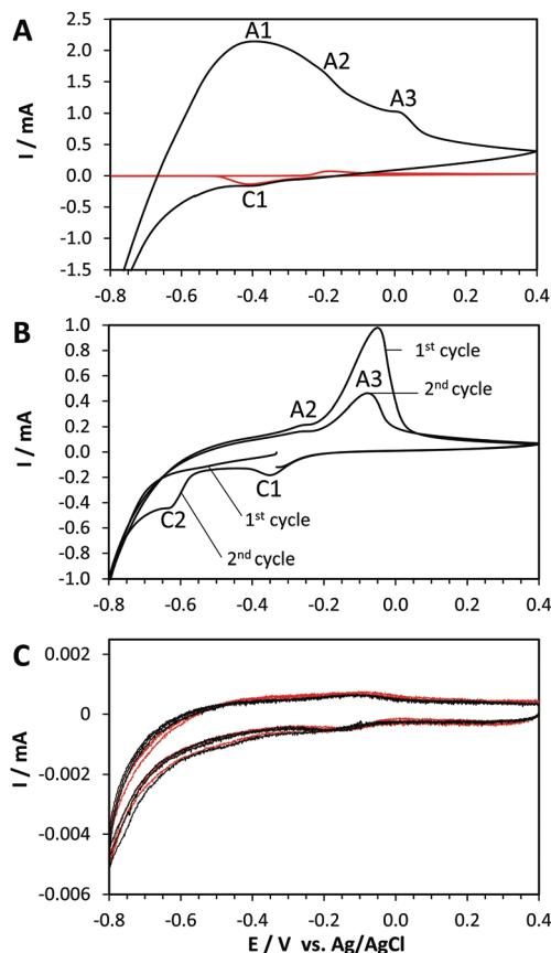
Fig. 2 Cyclic voltammograms of (a) the first cycle of n(\text{Fe}^{2+}\text{S}_n^{2-})_{(\text{s})} (formed from equimolar 11.4 mM \text{Fe}^{2+}_{(\text{aq})} and \text{S}_n^{2-}_{(\text{aq})} ) shown by the black trace and 11.4 mM \text{FeCl}_3 only by the red trace (for which the second voltammetric cycle is shown). (b) 5.7 mM \text{Na}_2\text{S}_{n(\text{aq})} and n(\text{Fe}^{2+}\text{S}_n^{2-})_{(\text{s})} (formed as above) in 200 mM \text{K}_2\text{HPO}_4 (pH 7), which shows both the first and second voltammetric cycle. Panel (c) depicts a voltammetric sweep of 0.5 mM \text{Na}_2\text{S}_{(\text{aq})} (red) and ca. 0.5 mM \text{Na}_2\text{S}_{n(\text{aq})} in a 100 mM \text{K}_2\text{HPO}_4 buffer (pH 7) (black). The scanning speed was 10 mV \text{s}^{-1} and the open circuit potential was the starting point for the potential sweep.
