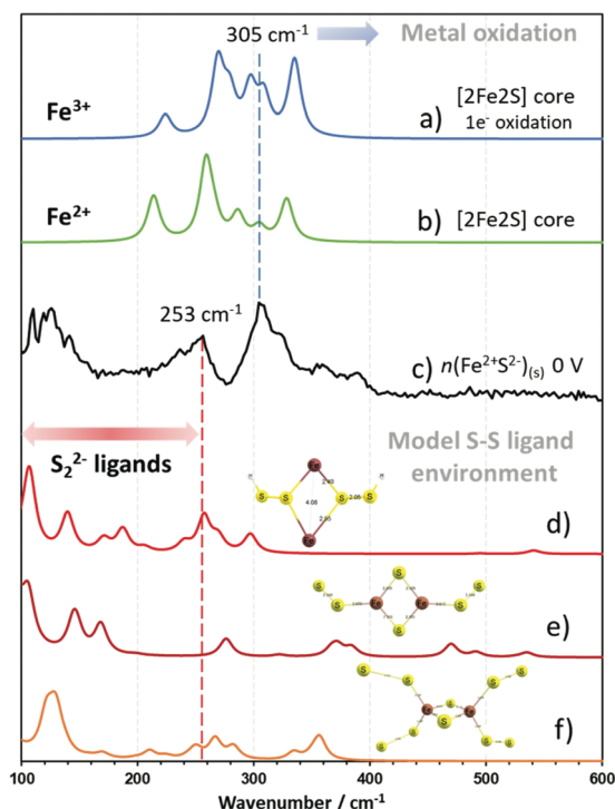
Fig. 6 Simulated Raman spectra of [2Fe-2S] cores from FeS nanoparticles and model persulfide ligand environments on the example of [2Fe-2S] clusters, in comparison to n(\text{Fe}^{2+}\text{S}^{2-})_{(s)} oxidized at 0 V. Spectra (a) and (b) correspond to core extracted [2Fe-2S] rhombs, where (a) depicts the blue-shifted Raman bands of a 1e^- oxidized 8(\text{FeS})_{(aq)} particle and (b) the non-oxidized, neutral charge 8(\text{FeS})_{(aq)} particle. Raman spectrum (c) depicts the measured spectrum of n(\text{Fe}^{2+}\text{S}^{2-})_{(s)} oxidized at 0 V, which was stored anaerobically for 2 months. Spectra (d) to (f) show the vibrational modes of persulfide ligated [2Fe-2S] clusters, where (d) corresponds to ^2[2\text{Fe}-(\text{SSH})_2]^{3+} , (e) to ^1\{[2\text{Fe}-2\text{S}](\text{S}_2^{2-})_2\}^{4-} and (f) to ^1\{[2\text{Fe}-2\text{S}](\text{S}_2^{2-})_4\}^{8-} .
