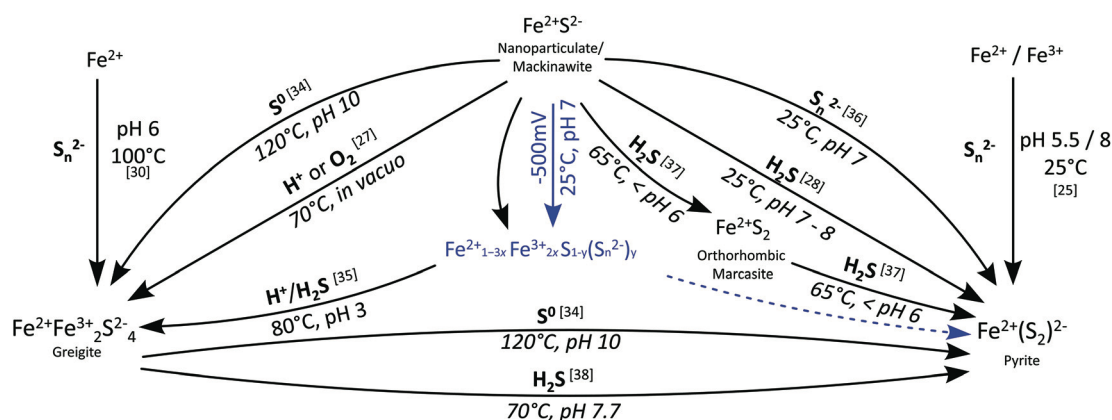
Fig. 1 Schematic overview of the known aqueous oxidation pathways of iron(II) sulfide/mackinawite to greigite, marcasite and pyrite. The oxidants employed or assumed in the respective reaction (and along with literature references) are displayed in bold; the pH and temperature of the reaction conditions are indicated below the oxidants. Indicated in blue is the reaction studied in this work, in which an iron sulfide phase (previously termed ferric iron containing mackinawite 35 ) was produced using an indium tin oxide electrode at -0.5 V vs. Ag/AgCl, pH 7. For a detailed review of mineral transformations of FeS, including higher temperatures, see ref. 17.
