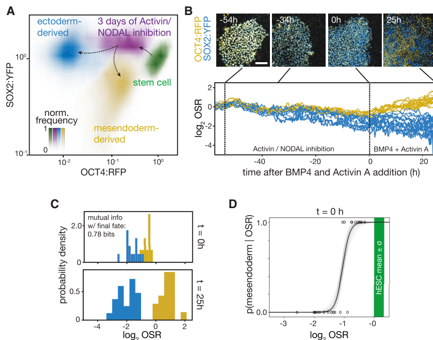
Figure 2. Dynamics of OCT4 and SOX2 accurately predict mesendoderm competence
