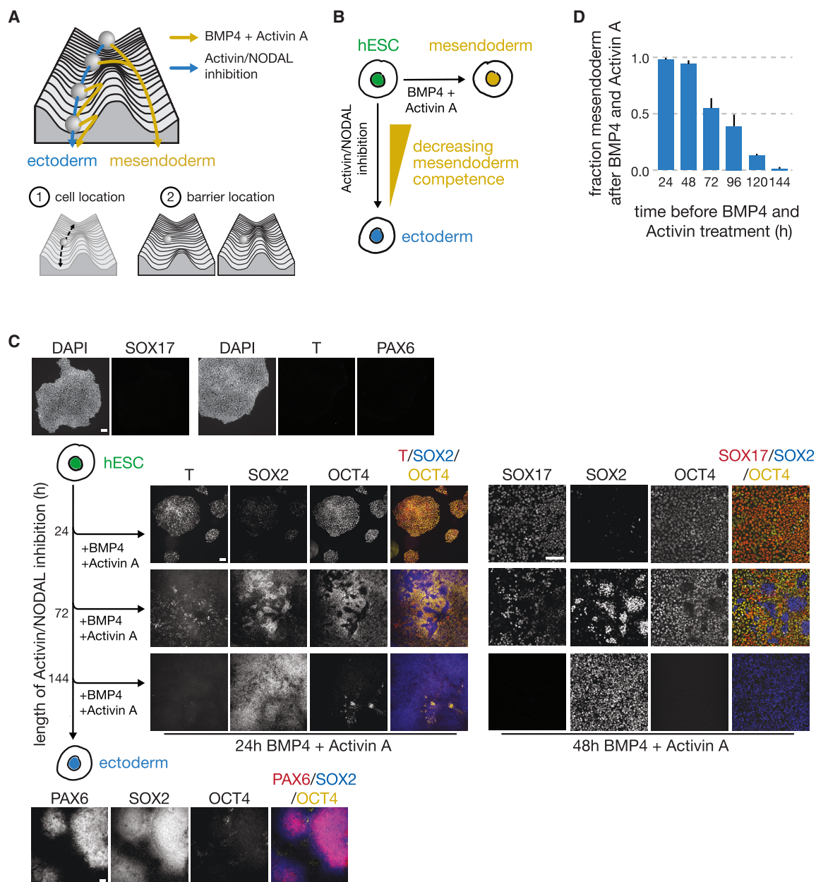
Figure 1. Stem cells lose competence to adopt mesendodermal fates upon BMP4 and Activin A signal exposure with increasing duration of activin/NODAL inhibition
