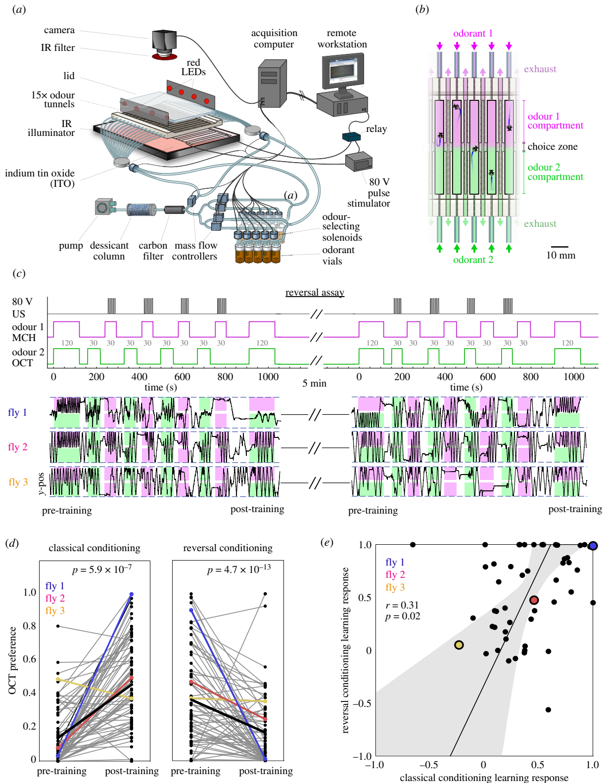
Figure 1. Individuality in associative learning. (a) Schematic of the reversal assay. (b) Zoom-in view of the linear behavioural arenas, with odorant flowing into each half. (c) Diagram of training protocol (top). Grey numbers indicate the length in seconds of each stimulus phase. Note that the timing of US delivery differs in the classical and reversal phases. Position in the arena versus time kymographs of three specific flies undergoing conditioning. Magenta and green shading indicate the portions of each arena that are filled with OCT and MCH, respectively. (d) Octanol preference of flies before and after training with MCH as the CS+ (left) and with OCT as the CS+ (right). Points are individual flies. Coloured examples correspond to the individual flies highlighted in (c). p -values reflect paired t -tests. Thick black line represents the mean. (e) Scatterplot of individuals' learning responses for reversal versus classical conditioning trials ( r = 0.31 ; p = 0.02 ; n = 53 ). Points are individual flies. Line is the best linear fit and shaded region is the 95% CI of the best-fit line.
