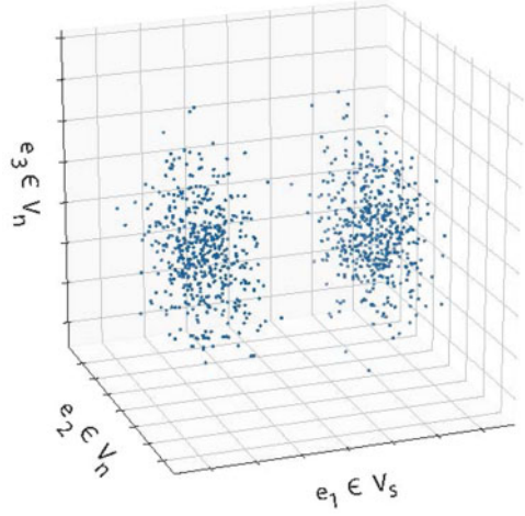
Fig. 1. Gaussian data with unit variance shown along three axes. The marginal distribution of \rightarrow e_1 contains signature of distinct clusters, with a bimodal marginal distribution where each mode corresponds to a cluster. Here, the clusters are linearly separable along the e_1 axis. The marginal distributions of \rightarrow e_2 and \rightarrow e_3 are unimodal, and do not linearly separate groups of data points. Here, we designate \rightarrow e_1 as part of V_s as it contains multimodal signal, and e_2, e_3 \in V_n do not. The three axes shown here represent a subspace of a D > 3 -dimensional distribution
