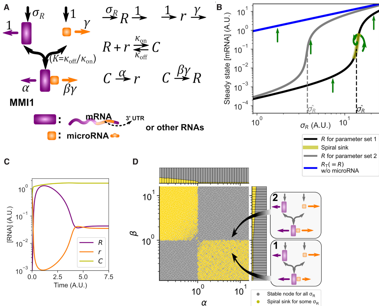
Figure 2. Dynamics of the MMI1 Model. (A) Left: illustration of reaction network of the MMI1 Model. Purple icon represents mRNA. Orange icon represents microRNA. Horizontal arrows represent degradation. Straight vertical arrows represent synthesis. Curved arrows represent binding. Right: eight chemical reactions associated with the MMI1 Model, which describes the dynamics of each molecular species with the law of mass-action (equation 1 and Supplementary Data Section 1). UTR, untranslated region. (B) Two representative signal-response curves (black and gray) showing steady state levels of R in response to transcription rate constant \sigma_R . Green arrows indicate the type of these steady states: straight arrows show stable nodes and spiral arrow shows spiral sinks. Blue curve shows the microRNA-free response for both parameter sets. (C) Time-course simulation showing transient oscillation near a spiral sink (parameter set 1). One time unit is approximately 1.44 \times t_{1/2} where t_{1/2} is the half-life of the mRNA. (D) Distribution of the parameter sets with spiral sink steady state (yellow, e.g. parameter set 1) and those without (gray, e.g. parameter set 2) in the space of two representative parameters (RDFs). Callouts illustrate the two representative parameter sets (same as those in B) with degradation rate constants represented by arrow lengths. Only the values of \beta differ between the two sets. Marginal distributions are shown in stacked bars.
