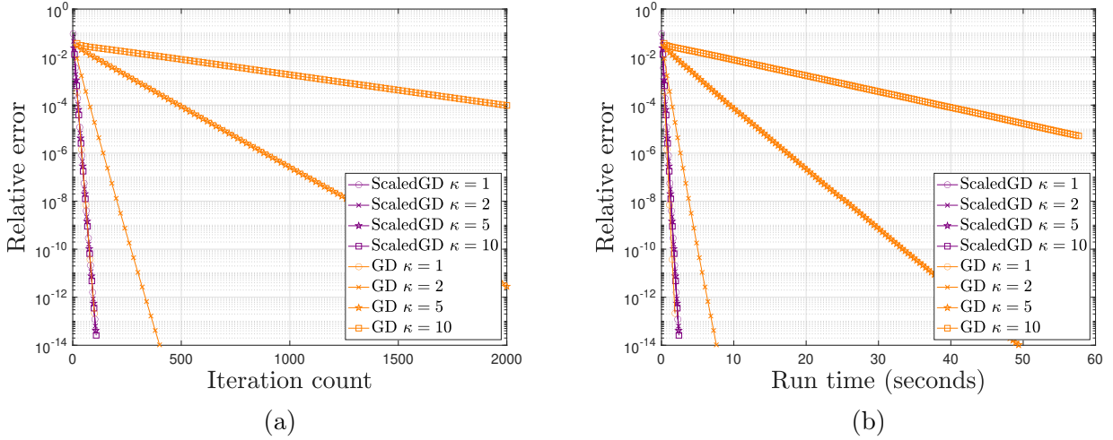
Figure 4: The relative errors of ScaledGD and GD with respect to (a) the iteration count and (b) run time (in seconds) under different condition numbers \kappa = 1, 2, 5, 10 for tensor completion with n = 100 , r = 5 , and p = 0.1 .
