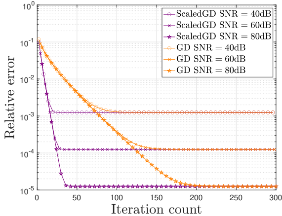
Figure 6: The relative errors of ScaledGD and GD with respect to the iteration count under signal-to-noise ratios SNR = 40, 60, 80dB for tensor completion with n = 100 , r = 5 , and p = 0.1 .
