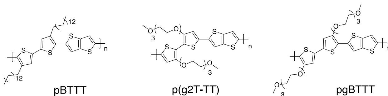
Figure 1. pBTTT, p(g2T-TT) and pgBTTT polymer structures
