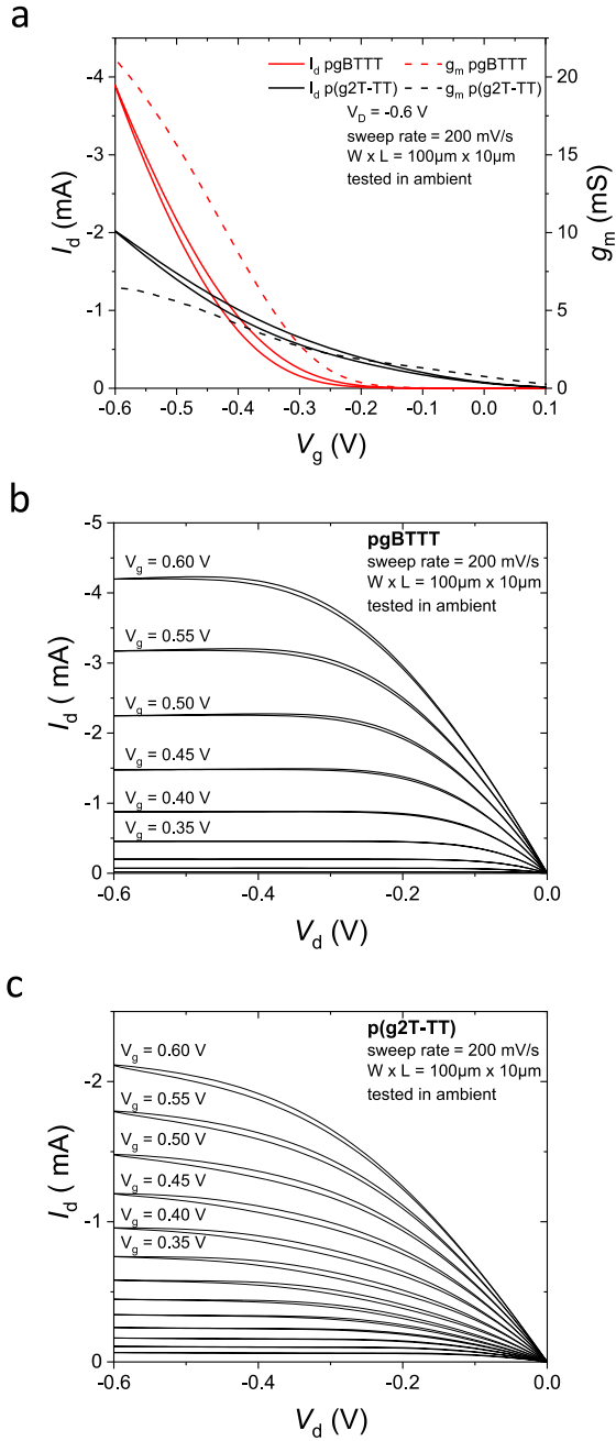
Figure 6. OECT Performance: (a) Transfer curves ( I_d vs V_g ) and voltage dependent transconductance ( g_m ) of representative pgBTTT and p(g2T-TT) devices, and output curves ( I_d vs V_d ) of the same (b) pgBTTT and (c) p(g2T-TT) devices.
