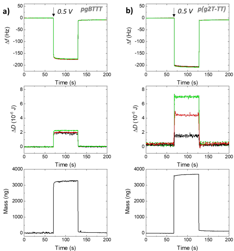
Figure 7. Frequency shifts ( \Delta f , top row), dissipation of energy ( \Delta D , mid row) and calculated mass shifts for a) pgBTTT and b) p(g2T-TT) polymer films cast on Au coated sensors, recorded in \text{NaCl}_{(aq.)} 0.1 M when a 60 s doping pulse at V = 0.5 V vs V_{OC} is applied. The overtones shown and chosen for the analysis are the 3 rd , 5 th and 7 th ; black, red and green solid lines, respectively.
