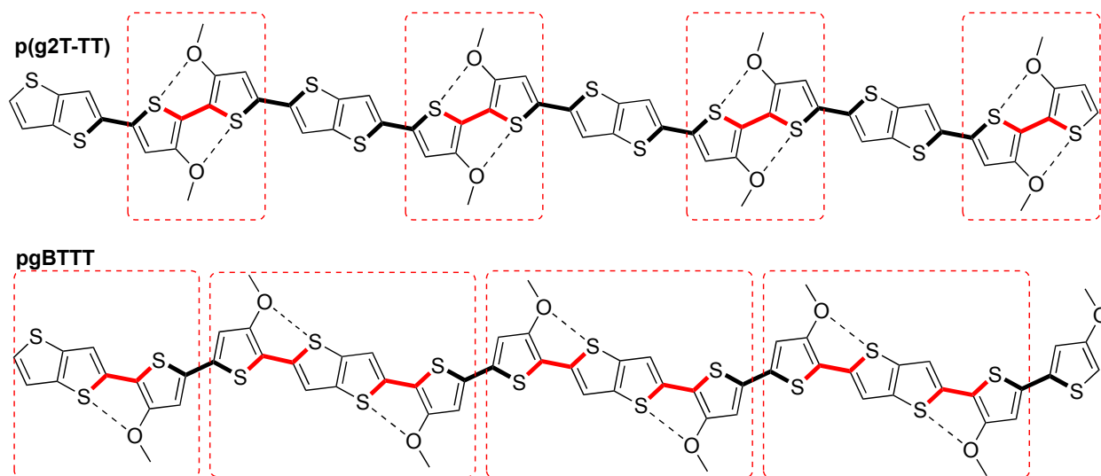
Figure 2. Sections of p(g2T-TT) and pgBTTT polymers highlighting S--O interactions (black dashed lines) leading to planarized dihedrals (bold red with \theta = 177 - 180^\circ ), and sections with twisted dihedrals in the absence of the S--O interactions (bold black with \theta = 154 - 156^\circ ). The red dashed squares highlight the planar sections in pgBTTT and p(g2T-TT). Geometries were optimized using \omega B97XD/6-31G* where \omega=0.1 Bohr -1
