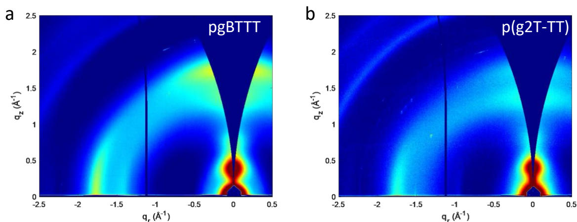
Figure 4. Two-dimensional grazing incidence X-ray q_r - q_z scattering map of (a) pgBTTT and (b) p(g2T-TT) thin films.
