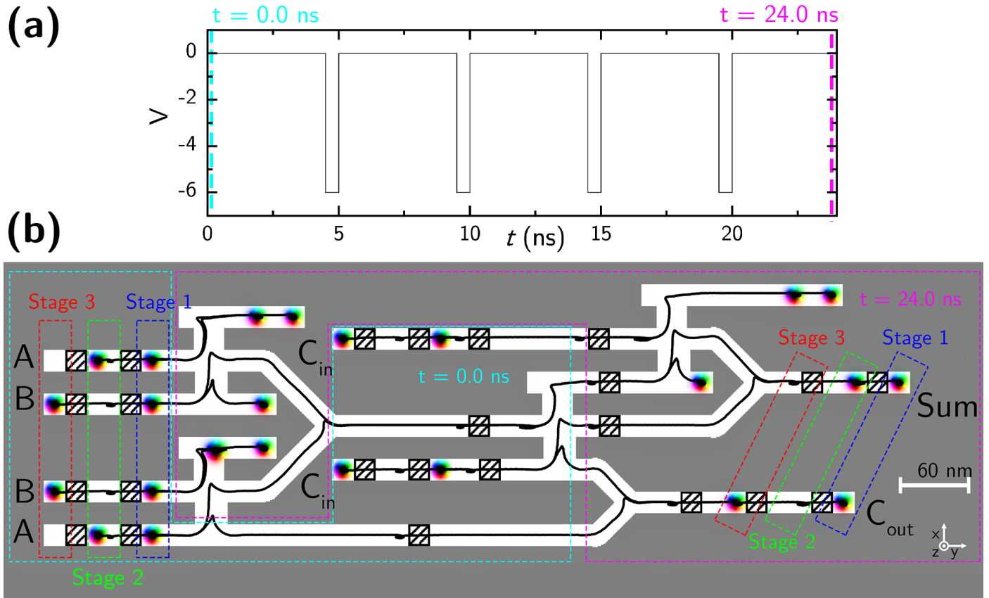
Fig. 5: VCMA synchronization of pipelined skyrmion one-bit full-adder with a constant current ( 5 \times 10^{10} \text{ A/m}^2 ) injected in the +y direction. (a) Clock waveform applied to the VCMA synchronizers (b) Micromagnetic simulation results for pipelined one-bit full-adder, demonstrating proper logical operation. Note that in a real system, the dead-ends would be replaced with out-of-plane tracks for cascaded logic.
