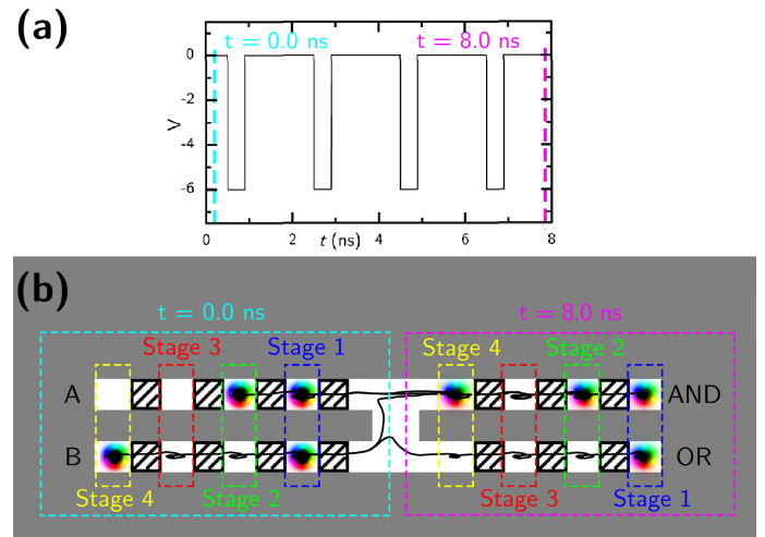
Fig. 4: VCMA synchronization of pipelined skyrmion AND/OR gate, with a constant current ( 5 \times 10^{10} \text{ A/m}^2 ) injected in the +y direction. (a) Clock waveform applied to the VCMA synchronizers (b) Micromagnetic simulation results for pipelined AND/OR gate, demonstrating proper logical operation.
