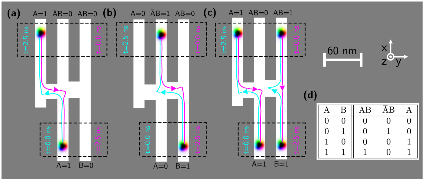
Fig. 6: Ressler-Feynman switch gate with current ( \pm 5 \times 10^{10} \text{ A/m}^2 ). Logic shown for input combinations (a) A=1, B=0 ; (b) A=0, B=1 , (c) A=1, B=1 . Skymion trajectory under positive and negative current is represented by cyan and magenta colored paths, respectively. The forward and reverse current trajectories vary slightly, demonstrating hysteresis. (d) Ressler-Feynman switch gate truth table
