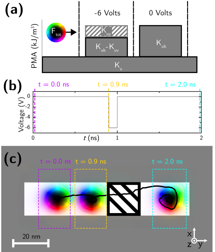
Fig. 3: VCMA synchronizer with a constant injected current of 5 \times 10^{10} \text{ A/m}^2 in the +y direction. (a) Illustration of the skyrmion synchronization method. The skyrmion is depinned when F_{tot} > K_{ub} + K_{uv} (b) Voltage applied to the VCMA region over one clock cycle. (c) Micromagnetic simulation results. Skyrmion trajectory is represented by the black line and the VCMA region is represented by the dashed square. The positive anisotropy barrier pins the skyrmion at t = 0.9 \text{ ns} and the negative voltage at t = 1.0 \text{ ns} reduces the barrier, depinning the skyrmion. At nonzero temperatures, the electric field must be larger than at 0 K to ensure pinning in the presence of noise [Walker 2021].
