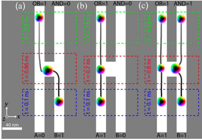
Fig. 2: Micromagnetic simulation results for AND/OR gate with current ( 5 \times 10^{10} \text{ A/m}^2 ) in +y direction, with skyrmion trajectory represented by the black path (a) A=0, B=1 (b) A=1, B=0 (c) A=1, B=1 . All simulations are performed with Mumax3 [Vansteenkiste 2014]. The SOT generated by the uniform electrical current was simulated as an external field to induce skyrmion motion. The Oersted field was excluded from the simulations, as its effect is insignificant relative to that of the Dzyaloshinskii-Moriya exchange interaction. Simulations were run at 0 K. Similar logic and system functionality is expected at nonzero temperatures, as both skyrmion transport and VCMA-based pinning are robust to thermal noise [Yu 2017], [Walker 2021], though correct operation may require adjustments to material composition, current distribution, and geometry.
