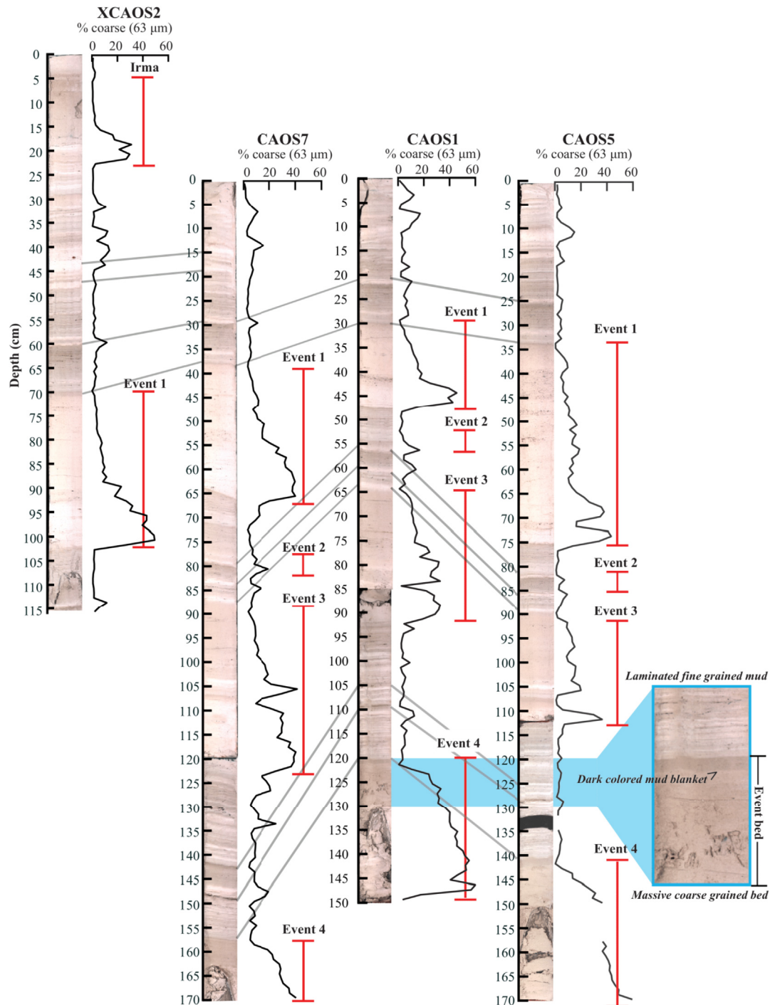
Fig. 2. Optical images from the ITRAX X-ray fluorescence scanner and coarse fraction ( >63 \mu\text{m} ) data of the shorter surface drives from XCAOS2 (collected in 2019) and CAOS7, CAOS1, and CAOS5 (collected in 2016). Visual event beds (Events 1–4) are denoted by the vertical red bars and labels. The top of Event bed 4 in CAOS1 is highlighted. Visual cues for event beds included: lighter colored sediments topped with darker colored sediment, visibly coarser grains, higher concentrations of organics, and no laminations. Lines of correlation (grey) are drawn between cores matching up the same sets of laminations in each core. XCAOS2 (far left) includes an event bed in the top 25 cm not found in any of the other 2016 cores that we attribute to Hurricane Irma in 2017. Inclined stratigraphy in the CAOS7 surface drive shown is not present in the longer drive and likely resulted from coring at a slight angle.
