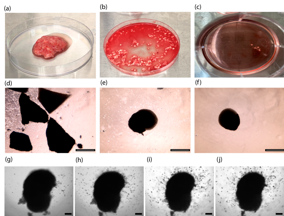
Figure 4. Development of GBOs from: (a) a tumor resected in the operating room coming as a bulk tumor, or (b) already dissociated in small pieces with a surgical blade until reaching less than 500 \mu\text{m} size. (c) Small pieces of tumor are forming GBOs after 15 days in the incubator. (d) GBOs are cut into small fragment pieces and incubated in media at t = 0 . (e) GBOs after t = 7 days in culture media and under permanent shaking. (f) GBOs after t = 15 days in culture media and under permanent shaking. GBOs embedded in a matrix to verify invasion properties for (g) 0 h, (h) 24 h, (i) 120 h, and (j) 168 h. Scale bar from (d) to (f): 1000 \mu\text{m} , obtained with \times 2.5 objective lens, under Evos microscope. Scale bar from (g) to (j): 200 \mu\text{m} , brightfield images were recorded on Cytation 5, using a 4\times objective lens.
