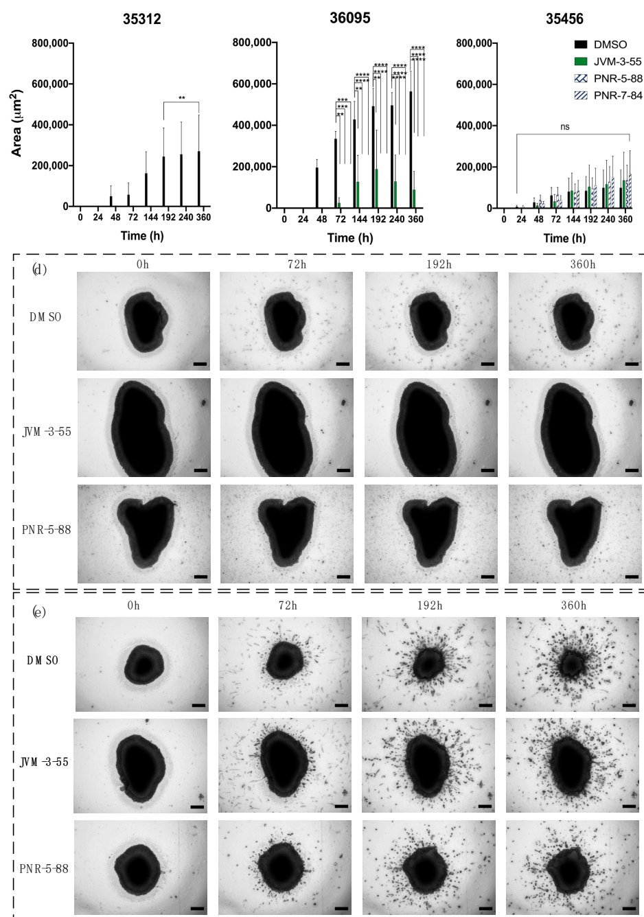
Figure 5. Evaluation of invasion ability of selected compounds on GBOs from different patients. The invasion was determined by automatic measurement of the area of cells invading into the matrix ( \mu\text{m}^2 ) in a function of the different times of incubation for patients (a) 35312, (b) 36095, and (c) 35456. The statistical analysis for significance was done using two-way ANOVA with the control (DMSO) for the different times of invasion as the comparative model with the Dunnett model, ns (non-significant) for adjusted p > 0.05 , ** for adjusted p \leq 0.01 , *** p \leq 0.001 , and **** p \leq 0.0001 . For each experiment, n = 3 . Brightfield images were recorded on Cytation 5 using a 4\times objective lens, in z-stacks of embedded GBOs in the matrix for 0, 72, 192, and 360 h with either DMSO, JVM-3-55, or PNR-5-88 for patients 36095 (d) and 35456 (e). Scale bar: 200 \mu\text{m} .
