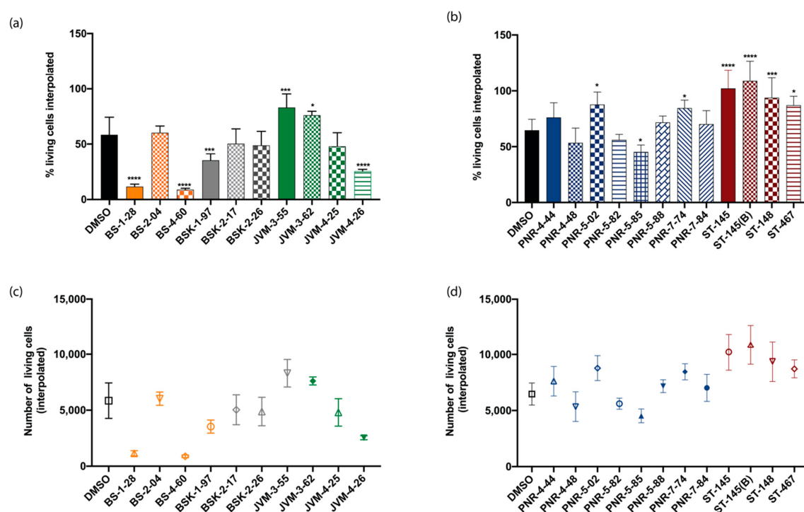
Figure 2. Determination of cytotoxicity on a U-251 MG cell 3-D model with percentage of living cells interpolated for (a) the first series of compounds tested: BS, BSK, and JVM, and for (b) the second series of compound tested: PNR and ST. Respective numbers of living cells interpolated for (c) the first series of compounds tested: BS, BSK, and JVM, and for (d) the second series of compounds tested: PNR and ST. Statistical analysis for significance determination was done using one-way ANOVA with the control (DMSO) as the comparative model with the Dunnett model, ns (non -significant) for adjusted p > 0.05 , * for adjusted p \leq 0.05 , *** p \leq 0.001 , and **** p \leq 0.0001 . For each experiment, n = 3 .
