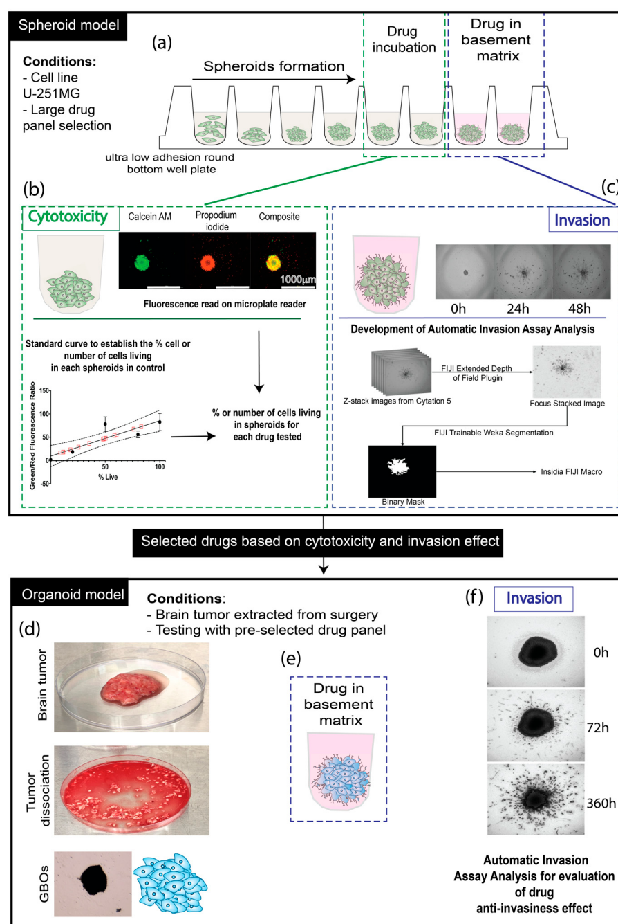
Figure 1. Schematic of experimentation. (a) U-251 MG cell spheroid formation in an ultra-low attachment round bottom well plate, followed by either drug incubation for cytotoxicity analysis or drug (10 \mu M) distributed in the basement membrane matrix Matrigel for invasion assay analysis. (b) Cytotoxicity assessment of the compounds on spheroids by interpolation of the standard curve established based on Calcein AM (green: living cells) and propidium iodide (red: dead cells) fluorescence intensity related to the known ratio of living/dead cells (0, 20, 50, 80, and 100%), with the establishment of a standard curve allowing us to interpolate (following mathematical model with Graphpad: Prism) (Figure S2) the percentage of living cells and also the number of cells related to the fluorescence intensity. (c) Development of an automatic invasion assay analysis using FIJI/ImageJ and INSIDIA macro. (d) Brain tumor extracted from surgery, followed by dissection and dissociation to constitute the GBOs. (e) Transfer of the GBOs in an ultra-low adhesion well plate with the drug incorporated in the basement matrix. (f) Evaluation of the invasiveness of the GBOs for 360 h maximum, using automatic invasion assay analysis.
