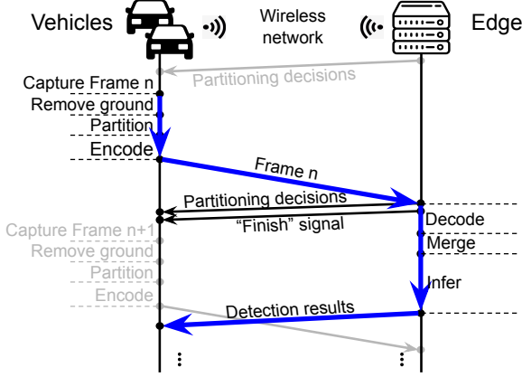
Figure 4: EMP Data Plane.
