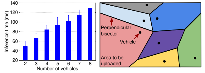
Figure 5: Inference time.
