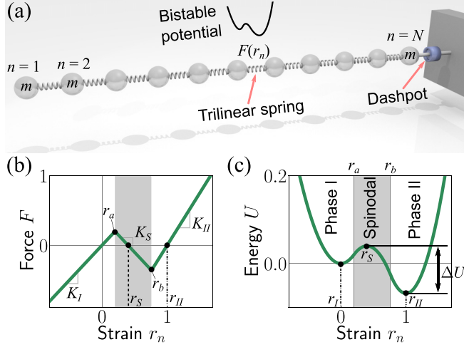
FIG. 1. (a) Schematic illustration of the system composed of bistable springs. The impact is applied to the leftmost unit ( n = 1 ) by setting an initial velocity. The rightmost mass ( n = N ) is connected to a dashpot. (b) The relationship between force and strain of a bistable spring is expressed by a trilinear function [cf. Eq. (1)]. The stiffness parameters are (K_I, K_S, K_{II}) = (1, -1, 1.5) and the strain parameters are (r_S, r_{II}) = (0.4, 1) . (c) The bistable energy landscape obtained from the trilinear force-strain relationship of panel (b).
