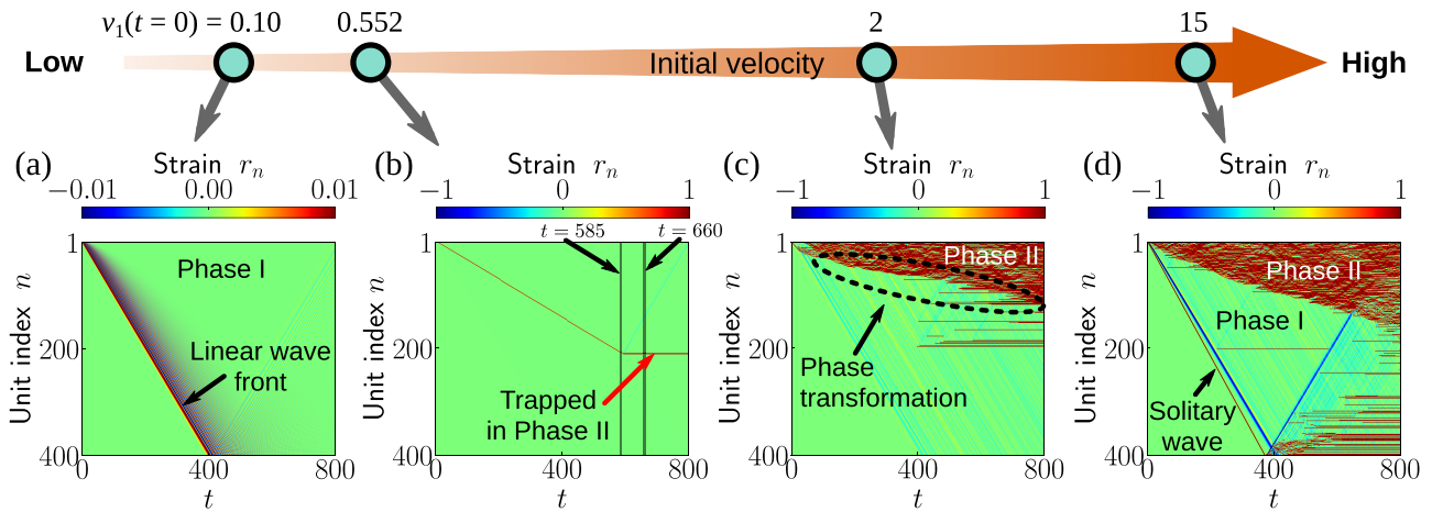
FIG. 2. Amplitude-dependent behavior for a bistable chain composed of strain-hardening springs ( K_{II}/K_I = 1.5 ). All unit cells are initially in Phase I. We apply an impact velocity to the first unit cell ( n = 1 ) by setting v_1(t = 0) \neq 0 . We consider four different values of the impact velocities: (a) v_1(t = 0) = 0.1 , (b) 0.552 , (c) 2 , and (d) 15 . The color indicates the strain r_n as a function of the unit index n and time t .
