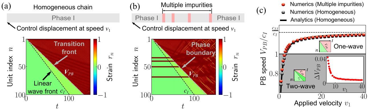
FIG. 13. Effect of multiple double impurities on phase transitions. Spatiotemporal plots for (a) a homogeneous chain (Phase I) and (b) a chain with double impurities ( K_{\text{imp}} = K_{II} = 1.5 ). We control the displacement of the first unit at constant speed v_1 = 1.2 . The gray (black) dashed lines indicate the phase boundary (linear wavefront). (c) We plot the speed of the phase boundary ( V_{PB} ) as a function of the applied speed v_1 . The inset shows the difference between the phase boundary speeds for the homogeneous chain without impurities and the chain with multiple impurities, which is defined as \Delta V_{PB} = V_{PB}^i - V_{PB}^h .
