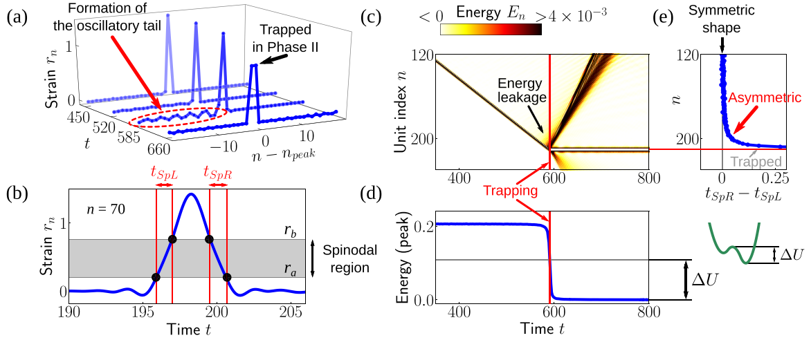
FIG. 3. Trapping behavior. (a) The spatial distribution of the subsonic wave packet generated by the impact velocity v_1(t = 0) = 0.552 is shown at different instants of time t . The waveforms for t = 585 and 660 correspond to the black vertical lines in Fig. 2(b), respectively. Each strain profile is shifted in the space domain so that the peak of the strain profile is located at n = 0 to ease visualization. (b) The strain change of n = 70 is shown as a function of time t . The shaded gray area indicates the spinodal regime [see also Fig. 1(c)]. To quantify the wave shape, we measure time widths in which the strain is in the spinodal region, t_{SpL} and t_{SpR} , bounded by the red vertical lines. (c) Surface plot of the energy E_n(t) = \frac{1}{2} m \dot{u}_n^2(t) + U_n(t) where U_n is the bistable potential-energy function of Fig. 1(c). Note that the colormap is adjusted for clarity of illustration of the energy leakage so that energies greater than 4 \times 10^{-3} all appear with a dark color. (d) The peak energy of the propagating wave packet is shown as a function of t . \Delta U is the energy barrier measured from the energy minimum in Phase II [see Fig. 1(c)]. The red vertical line indicates the trapping point at which the peak energy becomes lower than that of the energy barrier \Delta U . (e) We calculate the time difference t_{SpR} - t_{SpL} , which indicates the symmetric (if t_{SpR} - t_{SpL} = 0 ) or asymmetric waveform (otherwise).
