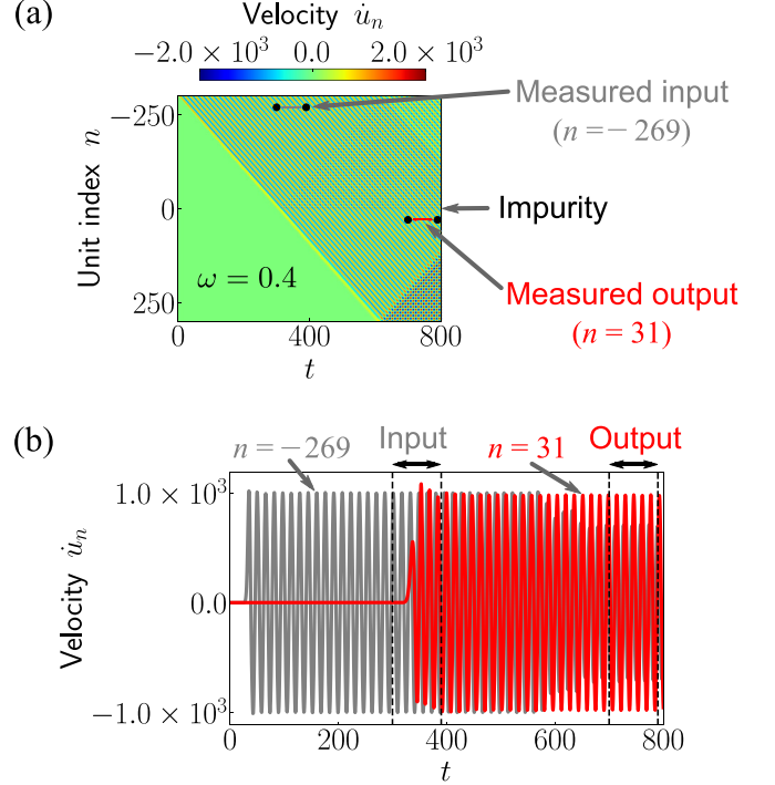
FIG. 11. Numerical simulations to obtain the transmission coefficient. (a) Spatiotemporal plot of velocity. We embed a single impurity (stiffness ratio \gamma = 0.5 ) in a chain composed of 601 units and apply a harmonic excitation ( \omega = 0.4 ) to the chain. (b) Temporal distribution of the velocity profiles v_n for (gray) n = -269 and (red) n = 31 .
