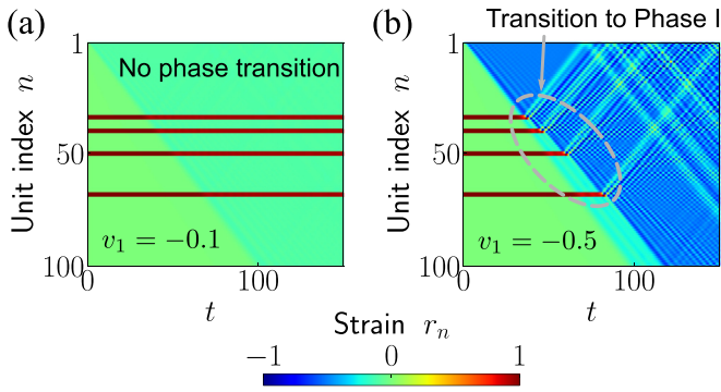
FIG. 14. A chain with multiple impurities under tension. To apply the tension, we control the displacement of the first particle at constant speed v_1 . Spatiotemporal plots of the strain wave profiles for (a) v_1 = -0.1 and (b) v_1 = -0.5 .
