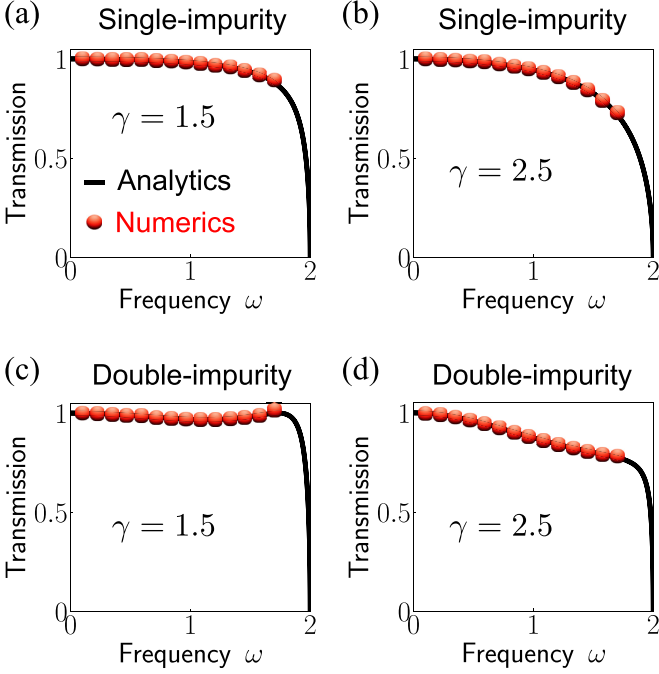
FIG. 12. Analytical transmission compared with numerical simulations for (a), (b) single-impurity and (c), (d) double-impurity cases. We calculate transmission coefficients for stiffness ratios (left) \gamma = 1.5 and (right) \gamma = 2.5 .
