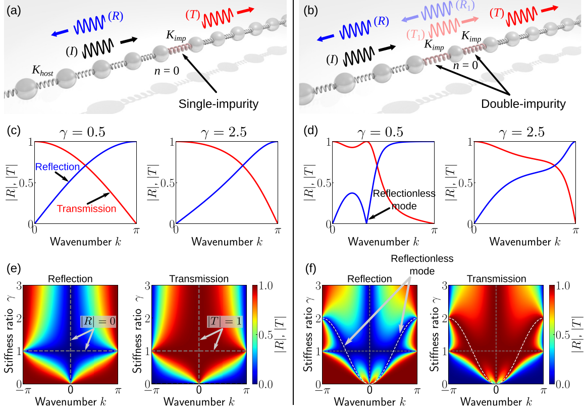
FIG. 4. Schematic illustrations for a chain with a (a) single and (b) double impurity. Analytical transmission and reflection coefficients for (c) single- and (d) double-impurity cases. The two different stiffness ratio cases (left) \gamma = 0.5 and (right) \gamma = 2.5 are shown. The reflection and transmission coefficients for (e) single- and (f) double-impurity cases are plotted as a function of stiffness ratio \gamma and wave number k . (e), (f) The gray dashed lines indicate |R| = 0 (or |T| = 1 ), and the reflectionless mode, which is expressed by Eq. (12), is denoted by the white dashed lines.
