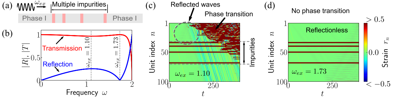
FIG. 8. Scattering by multiple double impurities. (a) The schematic illustration highlights the application of a harmonic excitation (with excitation frequency \omega_{ex} ) to the first unit ( n = 1 ) of the chain with multiple double impurities. The stiffness parameters for the host and impurities are K_{\text{host}} = 1 and K_{\text{imp}} = 1.5 , respectively. (b) The transmission and reflection coefficients for the double impurity with \gamma = 1.5 are shown as a function of frequency \omega . Surface plots of strain wave propagation are presented for (c) \omega_{ex} = 1.10 and (d) \omega_{ex} = 1.73 .
