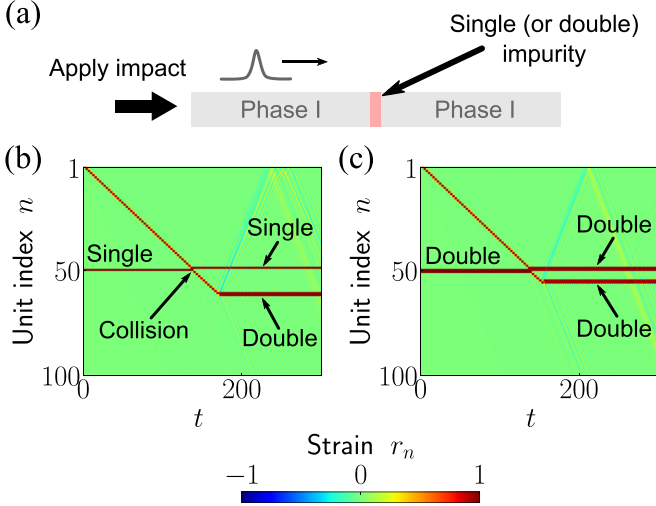
FIG. 6. (a) Schematic illustration of a collision of a propagating wave packet with an impurity. (b), (c) Spatiotemporal plots of strain wave profiles for the (b) single- and (c) double-impurity cases. We apply the initial velocity [ v_1(t=0) = 0.55 ] to the first particle to generate the subsonic propagating wave packet.
