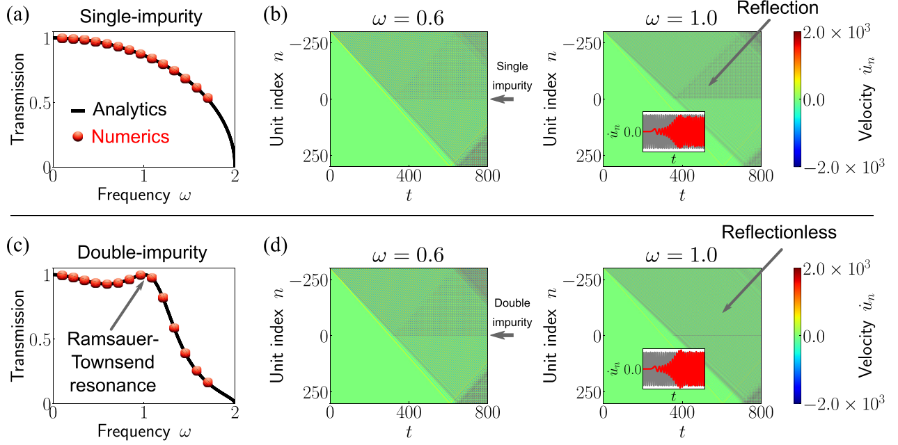
FIG. 5. Analysis of transmission. (a) Comparison between analytics (black line) and numerics (red markers) for a stiffness ratio of \gamma = 0.5 . (b) Spatiotemporal plots of velocity profiles for excitation frequencies of (left) \omega = 0.6 and (right) \omega = 1.0 , respectively. The inset shows the temporal dependence of the velocity \dot{u}_n for (gray) n = -269 and (red) n = 31 . (c), (d) Same as the top panels but for the case corresponding to a double-impurity chain.
