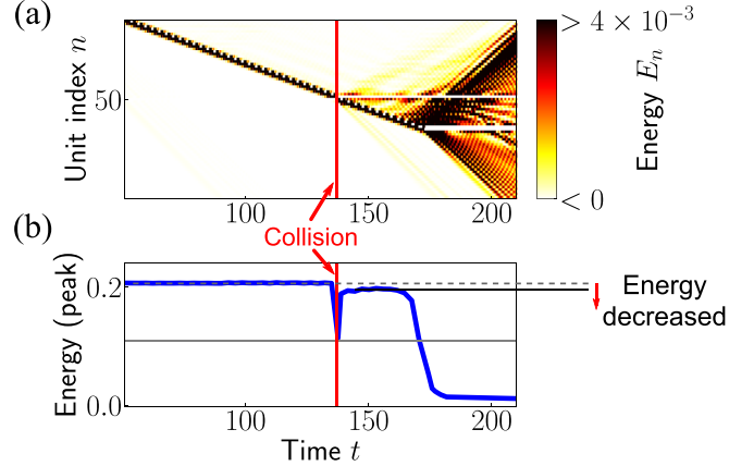
FIG. 7. Collision of a (subsonic) propagating wave packet with a single impurity. (a) Surface plot of the energy E_n(t) = \frac{1}{2} m \dot{u}_n^2(t) + U_n(t) where U_n is the bistable potential-energy function as shown in Fig. 1(c). The red vertical line indicates the collision point. (b) The peak energy of the propagating wave packet is shown as a function of time.
