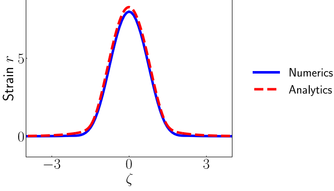
FIG. 10. Wave form analysis of the supersonic solitary wave. The blue solid line indicates the strain profile of the supersonic solitary wave with the wave speed of 1.076 obtained from the simulation [see Fig. 2(d)]. The red dashed line indicates the analytical solution based on the Padé approximation [Eq. (B5)].
