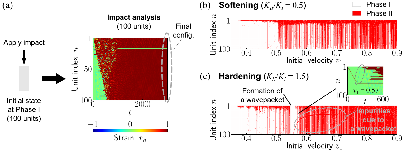
FIG. 9. Amplitude-dependent phase-transition behavior. (a) Schematic illustration for examining the steady-state configuration after an impact is applied to the chain. We extract the final configurations of the chain at t = 3000 and present them as a function of the impact velocity v_1 for (b) the softening ( K_{II}/K_I = 0.5 ) and (c) hardening ( K_{II}/K_I = 1.5 ) chains.
