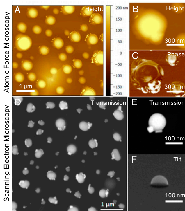
Fig. 1. AFM ( A and B ) height and ( C ) phase images demonstrating the unique morphology of the observed ammonium sulfate particles (15 September 2015 00:00 to 08:00 sample). SEM ( D ) transmission electron detector image (16 September 2015 00:00 to 08:00 sample), ( E ) transmission electron detector image (5 to 6 September 2015 16:00 to 00:00 sample) and ( F ) secondary electron detector 75^\circ tilted image (7 September 2015 00:00 to 08:00 sample) further demonstrating the morphology of these particles. All sample times are given in Alaska Daylight Time.
