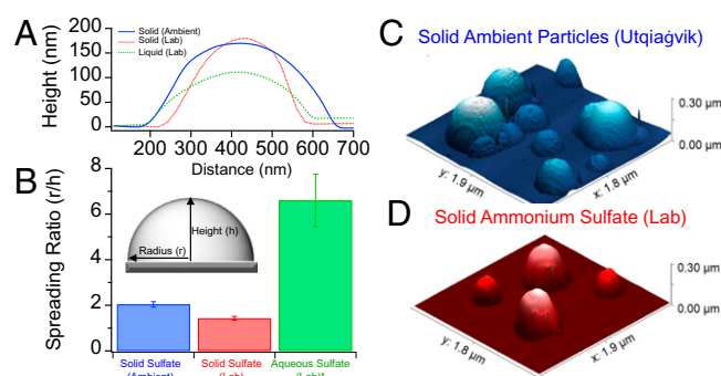
Fig. 2. ( A ) Average AFM height traces for ambient ammonium sulfate-dominant particles (16 September 2015 00:00 to 08:00 Alaska Daylight Time sample) (blue), as well as solid (red) and liquid (green) ammonium sulfate particles generated in the laboratory. Liquid ammonium sulfate plus sulfuric acid particles (green) are from Olson et al. (18). ( B ) Spreading ratios (radius/height) from AFM for ambient, solid (laboratory), and liquid (laboratory) (70, 72, and 25 particles measured, respectively) following method in Olson et al. (18) with error bars at 95% confidence interval. The inset cartoon shows how radius and height are defined for calculating the spreading ratio. AFM three-dimensional height profiles for ( C ) ambient ammonium sulfate-dominant particles from Utqiagvik and ( D ) solid laboratory-generated ammonium sulfate particles.
