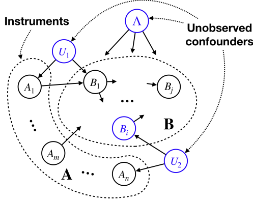
Figure 2: Illustration of a general IV model. Unobserved variables are shown in blue. The variables in \mathbf{B} are all children of \Lambda . The variables in \mathbf{A} are referred to as instruments, must be observed, and cannot be children of \Lambda .
