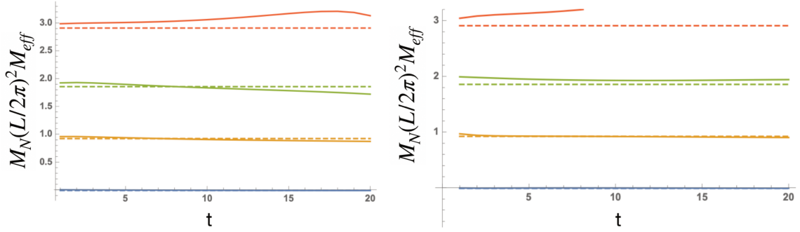
Figure 4: Effective masses for the two-nucleon system for the scattering phase shift shown in Fig. 1 (no physical bound state) using two-nucleon operators spatially displaced by \Delta = 1 (left) and \Delta = 5 (right) at the source and momentum space operators at the sink. The exact spectrum is shown as a set of dashed lines.
