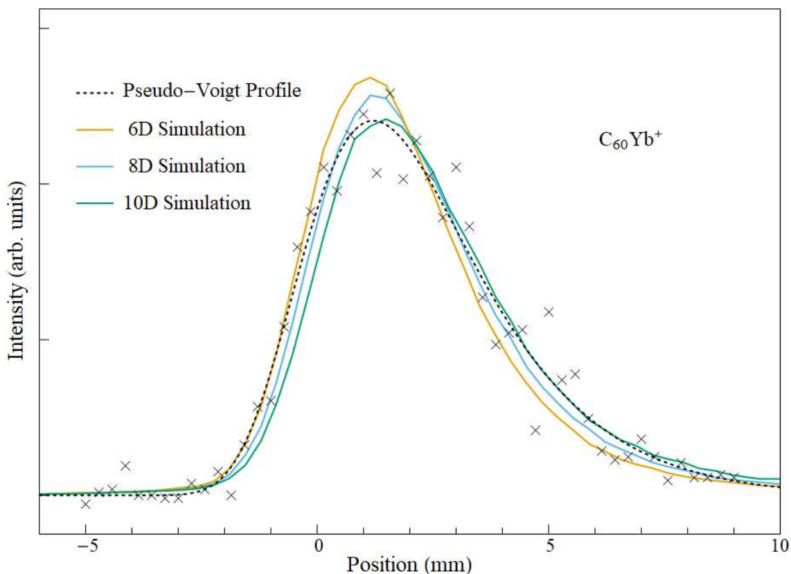
Figure S2. The crosses are beam deflection data points for nanodroplets containing C_{60}Yb , and the dashed line is a smoothing fit to these points using an asymmetric pseudo-Voigt function. The colored lines are the results of Monte Carlo simulations assuming three different values of the dipole moment of the complex and a dopant ionization probability parameter \gamma = 0.12 .
