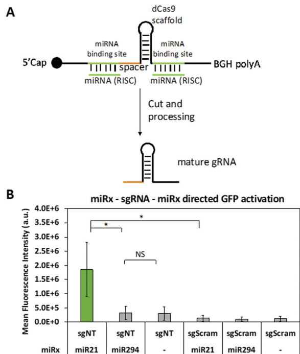
Fig. 1 (A) Depiction of miR-inducible CRISPR/Cas9. A pre-gRNA is flanked by two miR binding sites. After specific miR binding, mature gRNA is formed by RISC-mediated cleavage. (B) Confirmation of miR-sgRNA-miR behavior in HeLa cells. Only highly expressed miR21 was able to induce processing and gRNA activation. No difference in GFP expression was observed when miR294 was used or when sgNT was expressed directly from a CMV promoter or when scrambled gRNA (sgScram) was used as a negative control. Data are the average of three or more biological replicates (separately transfected wells), and the error is the standard deviation (SD) of the mean. * p < 0.05 , ** p < 0.01 , *** p < 0.001 , NS = no statistically significant difference.
