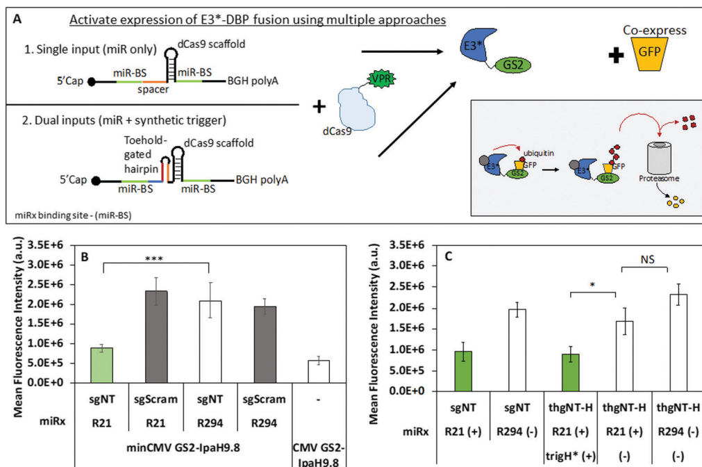
Fig. 4 (A) Conditional protein degradation based on induced expression of a specific ubiquibody (E3*-DBP). Expression of E3*-DBP is conditionally upregulated when either (1) a native miR is used to correctly process sgRNA in the cytosol or (2) both a native miR and a cytosolic RNA trigger are used to activate thgRNA. (B) miR-directed conditional protein degradation. We observed 62% knockdown of GFP using this strategy as compared to 76% knockdown using sgRNA expressed from a hU6 promoter. (C) Conditional GFP degradation using an AND gate (miRx and synthetic trigger (trigH*)) design to activate GS2-lpaH9.8 expression. When both inputs are present (miR21 and trigH*) to activate thgRNA properly, we observed 62% knockdown of GFP, while minimal degradation was detected in the presence of only one of the two processing steps. Data are the average of three or more biological replicates (separately transfected wells), and the error is the standard deviation (SD) of the mean. * p < 0.05 , ** p < 0.01 , *** p < 0.001 .
