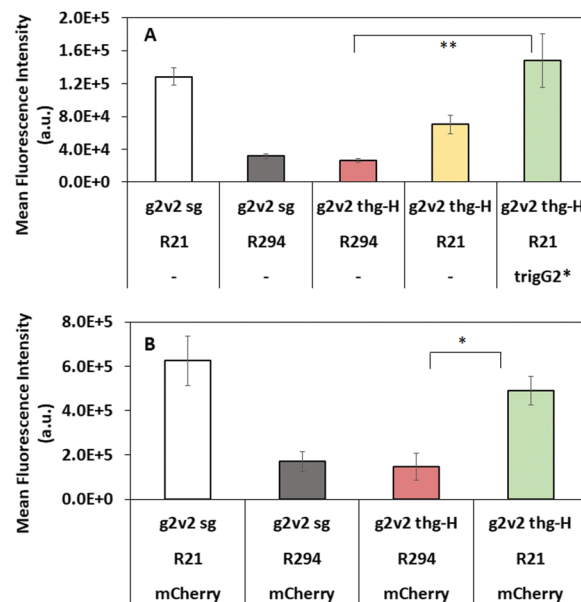
Fig. 3 Extending the miR-gated thgRNA design to target mCherry mRNA. (A) A synthetic trigger was first used to evaluate the design. We observed a leak of 36% in the presence of miR21 and a fold change of 2.1 in the presence of both inputs (miR21 and trigG2*). (B) The use of full-length mCherry mRNA as the trigger. Activation was detected only when both miR21 and mCherry mRNA were presented. Data is the average of three or more biological replicates (separately transfected wells), and the error is the standard deviation (SD) of the mean. * p < 0.05 , ** p < 0.01 , *** p < 0.001 .
