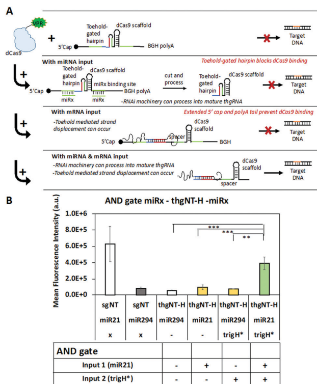
Fig. 2 (A) Schematic of the AND gate architecture using miR and mRNA as dual inputs. Both inputs are required (miR21 and mRNA) for proper processing of the 5' and 3' ends and to unblock the spacer region. The activated miR-gated thgRNA can complex with dCas9 for targeted up-regulation of GFP expression. (B) Induced GFP expression using the AND gate designs (miR-thgNT-H-miR). We observed negligible leak when neither input or only a single input was present (miR21 or thgH*) but observed a 7-fold increase when both inputs were present (miR21 and thgH*). Data are the average of three or more biological replicates (separately transfected wells), and the error is the standard deviation (SD) of the mean. * p < 0.05 , ** p < 0.01 , *** p < 0.001 .
