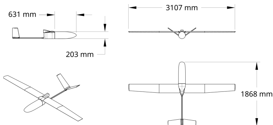
Figure 2. Overview of the S2 fixed-wing aircraft.
