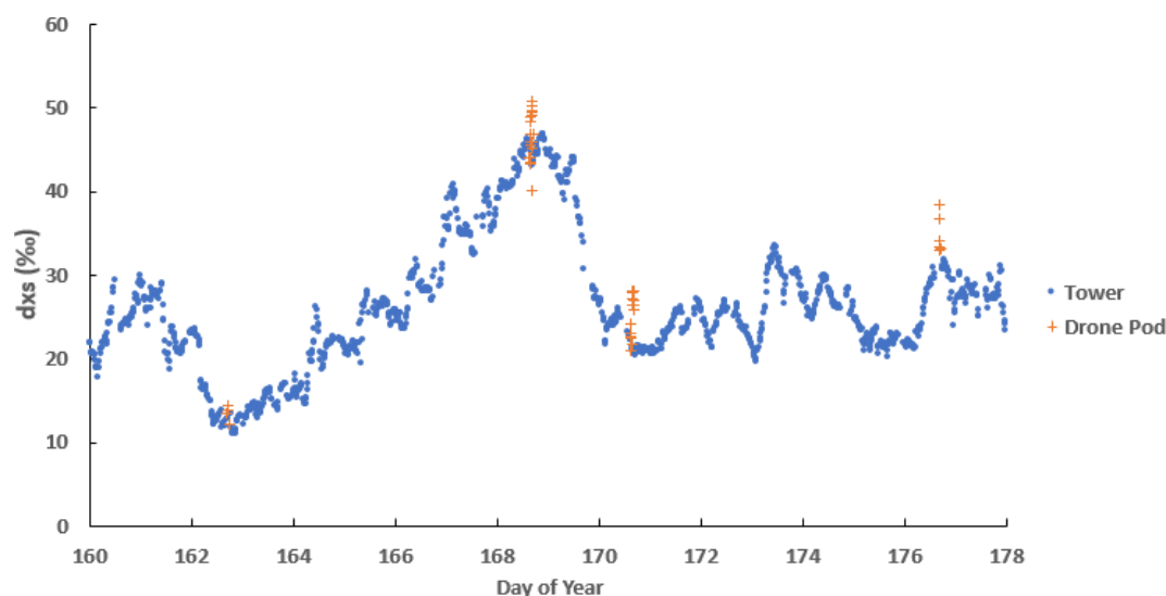
Figure 5. Comparison in second-order parameter dxs between the tower setup present at the EastGRIP camp in 2019 and 2 m pod intercomparison measurements. Drone pod measurements on 163 DOY (day of year) and 176 DOY correspond to flask measurements taken at 2 m during a flight mission. All measurements from both tower and UAV are tied to the same isotopic water standards listed in Table 1.
