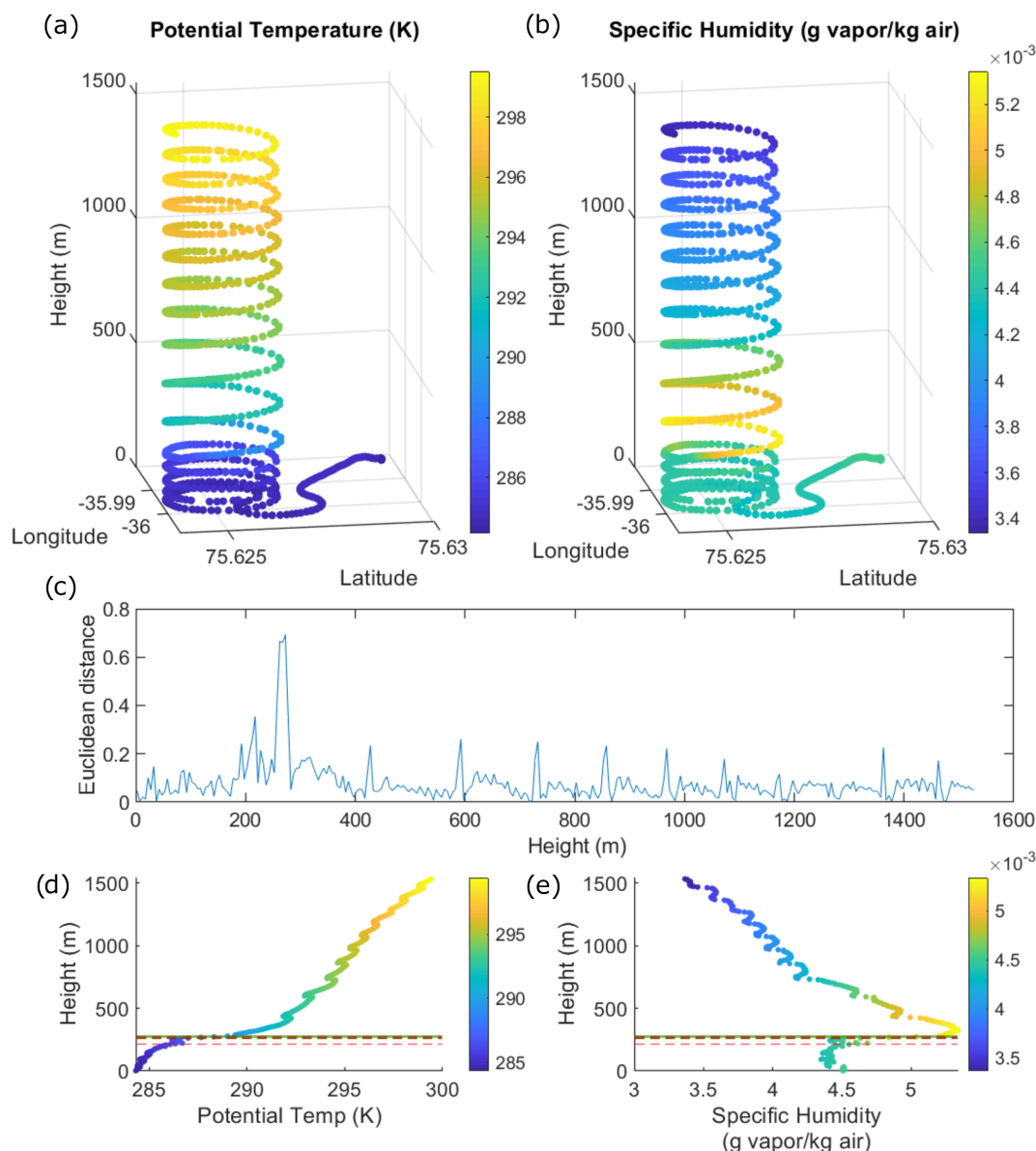
Figure 7. The ascension profile for the 12 June flight mission available to the operator to determine PBL location. The flight path reached a maximum altitude of \sim 1500 m a.g.l. ( a and b ). The potential candidate for the Euclidean distance determination of the PBL is shown to be at approximately 272.5 m a.g.l. ( c ). The top three candidates for PBL all correspond to approximately the same location (green and dotted lines d–e ). There is a modest gradient in potential temperature over the flight path of about 16^\circ\text{K} ( d ). Specific humidity shows an inversion in the first few hundred meters of flight at the determined location of the PBL ( e ).
