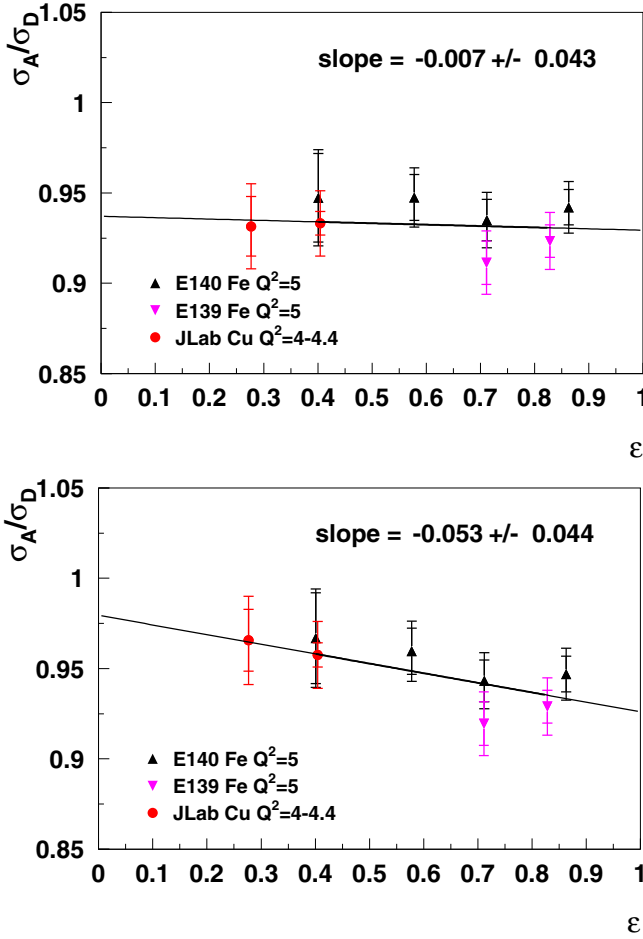
FIG. 22. Extracted cross-section ratios using the updated data from Refs. [16,107] and E03103 experiment as a function of \epsilon for the Fe/Cu targets for x = 0.5 and Q^2 values as mentioned in the legend. The top (bottom) plot shows the target ratio without (with) Coulomb corrections applied. Inner error bars denote statistical and point-to-point uncertainties combined in quadrature while outer error bars include contributions from normalization uncertainties. The uncertainty on the slope is calculated from point-to-point errors as well as the experiment-dependent normalization uncertainties.
