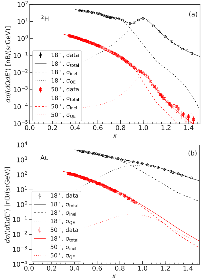
FIG. 6. Data and model cross section for ^2\text{H} and ^{197}\text{Au} at selected kinematics. Here, the circles show 18 degree data and the squares show 50 degree data. Relative contribution from inelastic (dashed line) and quasielastic (dotted line) to the total cross section (solid line) are also shown in the figure.
