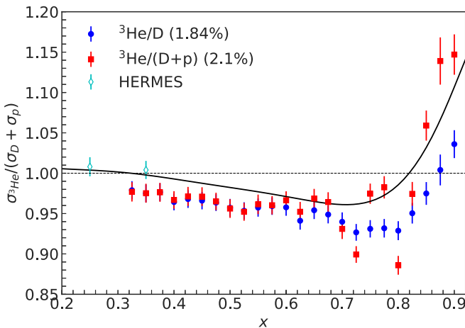
FIG. 19. Comparison of the isoscalar-corrected ^3\text{He}/\text{D} ratio (blue circles) to ^3\text{He}/(\text{D} + \text{p}) (red squares). The agreement is very good below x = 0.65 (which corresponds to W \approx 1.9 GeV). At larger x , the resonance structure in the free proton is evident.
