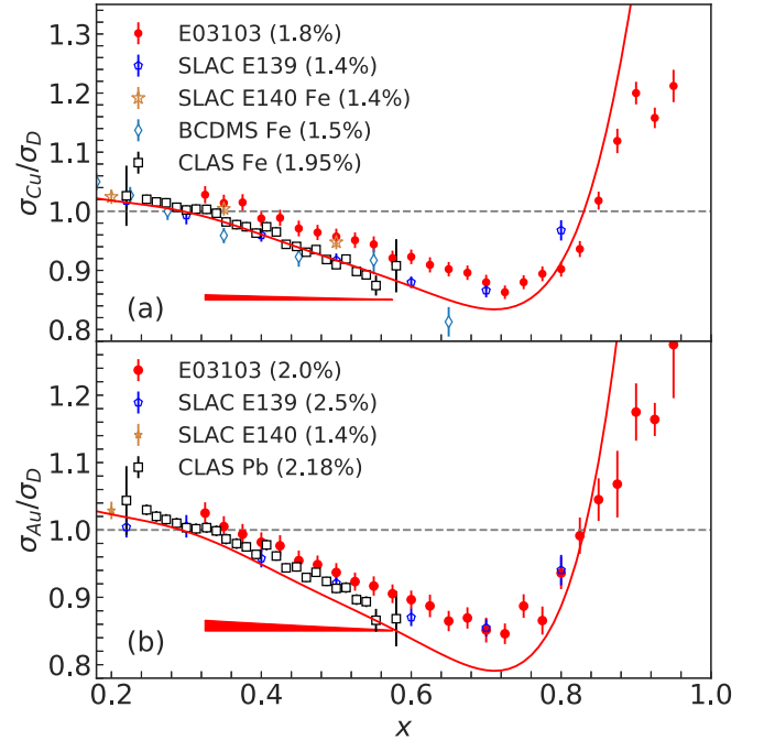
FIG. 20. EMC ratios for Fe and Cu (a) and for Au and Pb (b) as a function of x for the 40 degree data. Uncertainties are as described in Fig. 17. The SLAC E139 and E140 data include updated Coulomb and isoscalar corrections, while the CLAS data has been updated with isoscalar corrections only since Coulomb corrections had already been applied. BCDMS [108] Fe results are shown as published.
