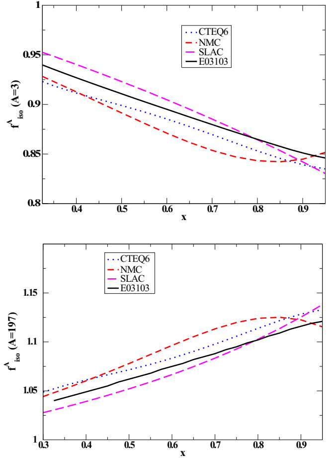
FIG. 12. Magnitude of isoscalar corrections for ^3\text{He} (top) and Au (bottom) targets for the 40 degree data for the different parametrizations of F_2^n/F_2^p as discussed in the text. The solid black line represents the multiplicative correction factors obtained using the smearing method discussed in the text and was used in the E03103 analysis for the EMC ratio extraction.
