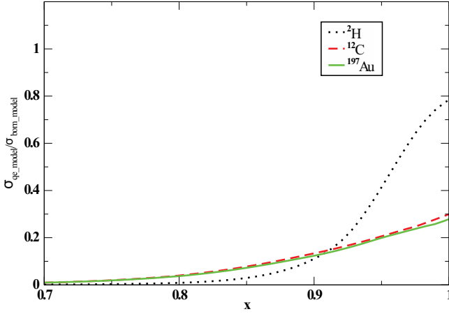
FIG. 13. Fractional quasielastic contribution to the cross section based on our model at 40 degrees for ^2H , ^{12}C , and ^{197}Au . Here, \sigma_{qe} is the contribution from the quasielastic piece of the model (in the Born approximation) and \sigma_{Born} is the total Born cross section.
