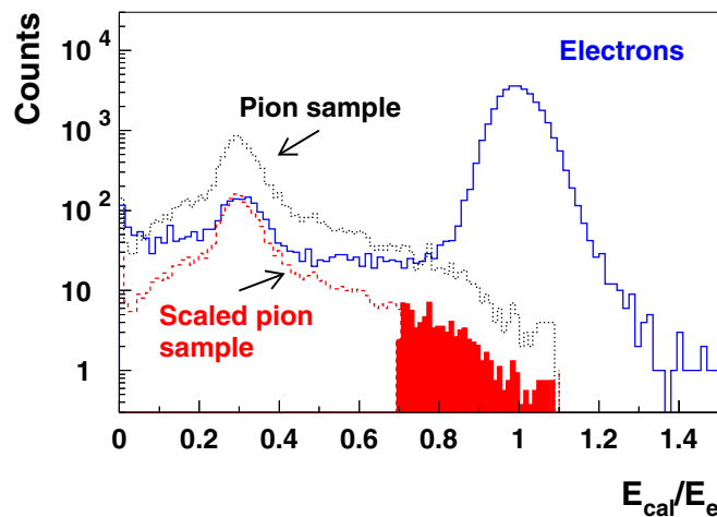
FIG. 5. Illustration of the extraction of pion contamination using calorimeter spectra. A pion data sample (black dotted curve) is renormalized to the number of counts in an electron data sample (blue solid curve) at low E_{\text{cal}}/E' . The resulting spectrum (red dashed curve) is then used to estimate the pion contamination in the region E_{\text{cal}}/E' > 0.7 (solid red).
