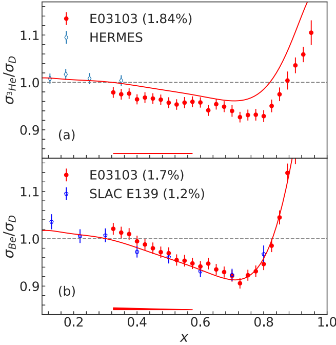
FIG. 18. Isoscalar EMC ratios for ^3\text{He} (a) and ^9\text{Be} (b) for the 40 degree data. Uncertainties are as described in Fig. 17. Also shown are the HERMES ^3\text{He} data [20,21] (updated to include our modified isoscalar correction). The solid curve shows an A dependent parametrization [16] for the EMC effect.
