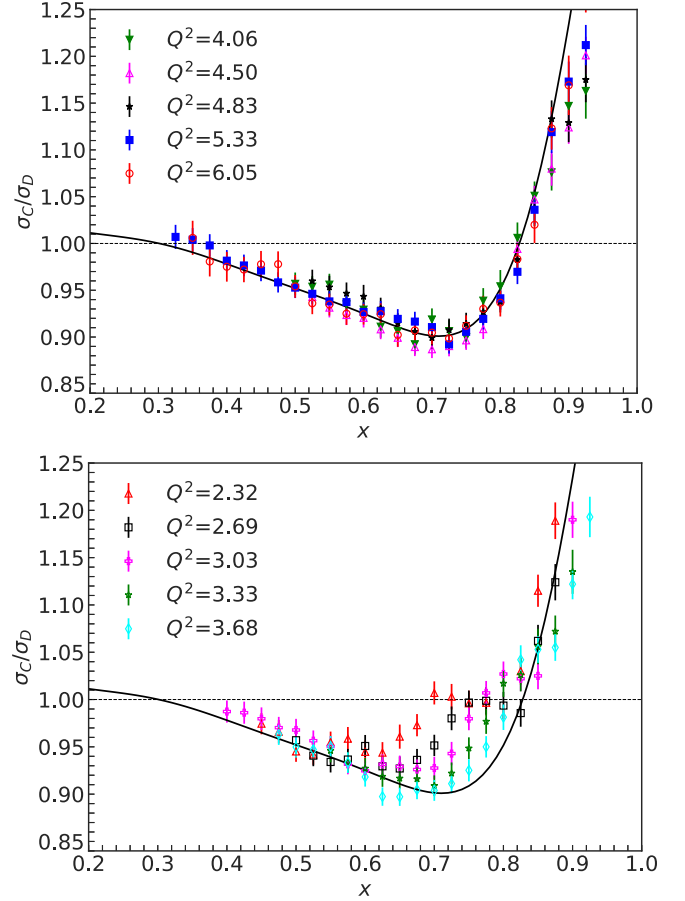
FIG. 15. Ratio of C and ^2\text{H} cross sections for the five largest Q^2 (top panel) and five lowest Q^2 (bottom panel) settings as a function of x . Uncertainties are the combined statistical and point-to-point systematic. The Q^2 values quoted are for x = 0.75 , and the data labeled Q^2 = 5.33 correspond to our primary results, taken at 40^\circ . The solid black line is the SLAC parametrization of the EMC effect for carbon [16].
