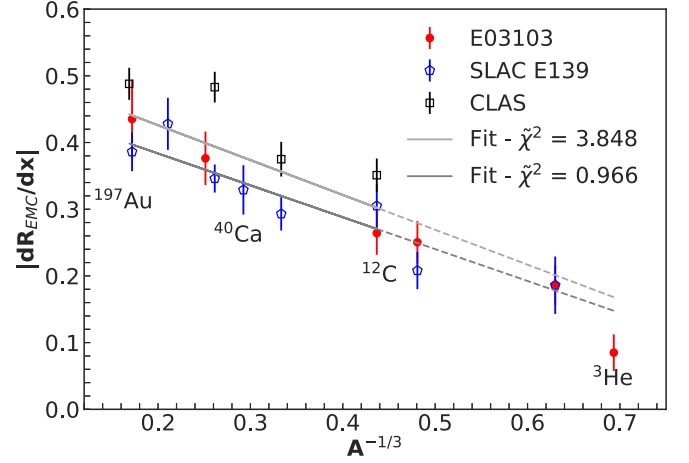
FIG. 23. EMC slope vs A for JLab E03103 (this work), SLAC E139 [16], and CLAS [104]. The linear fit excludes A < 12 nuclei, with the upper fit (and reduced \chi^2 value including all data sets), and the lower excluding the CLAS data.
