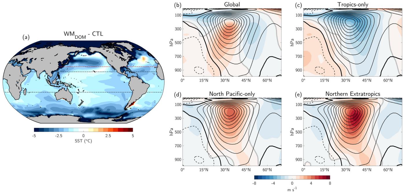
Fig. 6. North Pacific zonal wind response in WM SST . (a) Global SST anomalies (°C) for WM DOM minus CTL averaged during December–February. (b)–(e) Latitude–height cross-section of boreal winter (December–February) zonal wind anomalies (shading; \text{m s}^{-1} ) zonally averaged over the Pacific basin ( 120^\circ\text{E} – 110^\circ\text{W} ). Anomalies are from the WM SST CAM5 simulations forced with WM DOM SSTs (b) globally, (c) in the tropics-only ( 20^\circ\text{S} – 20^\circ\text{N} ; equatorward of dashed black lines), (d) in the North Pacific-only ( >30^\circ\text{N} ; poleward of red dashed line in North Pacific), and (e) in the Northern Hemisphere extratropics ( >30^\circ\text{N} ; poleward of the red dashed line at all longitudes). Black contours in (b)–(e) denote the winter WM SST control zonal wind climatology for this region. Solid (dashed) black contours denote positive (negative) values. Black contour interval is 5 \text{ m s}^{-1} , with the thick black contour marking 0 \text{ m s}^{-1} . Thick gray contour marks the 0 \text{ m s}^{-1} zonal wind anomaly contour.
