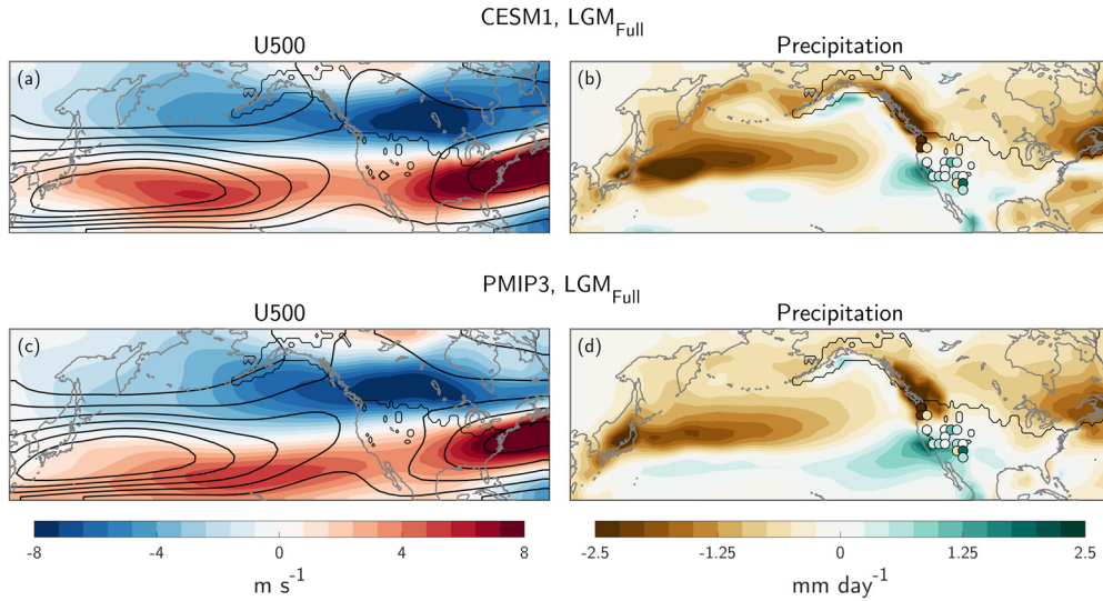
Fig. 2. North Pacific climate at the Last Glacial Maximum. Difference maps of LGM_{Full} minus CTL (a) 500 mb zonal wind (U500; m s^{-1} ) and (b) precipitation ( mm day^{-1} ) averaged during boreal winter (December–February). Thick black contours in (a) show wintertime U500 climatology in the pre-industrial control (contour interval is 5 m s^{-1} with max value of 30 m s^{-1} ). (c)–(d) As in (a)–(b), but for the ensemble mean of seven PMIP3 models forced with full LGM boundary conditions minus their respective pre-industrial control simulations. Thin black contour in each panel marks approximate ice sheet edge at the LGM. Filled circles in (b) and (d) show precipitation changes from proxy estimates (Table S2).
